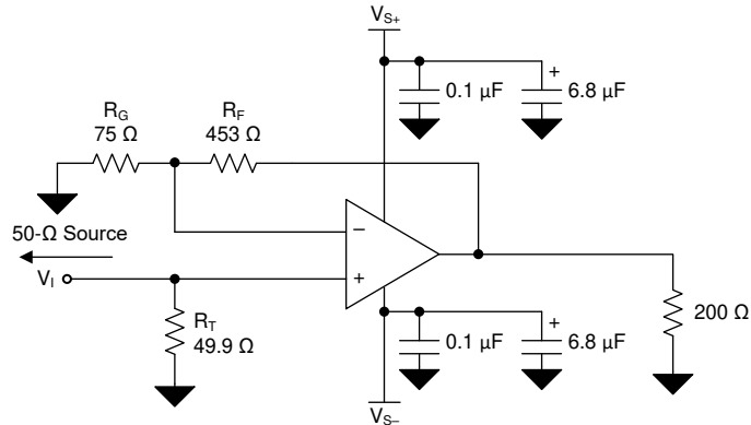
Figure 9-8. Split and Single Supply Circuit Configuration
