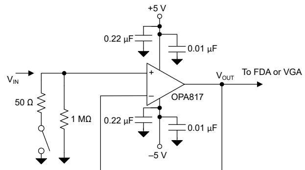
Figure 8-2. High Input Impedance DAQ Front-End
