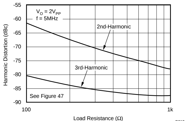
5 MHz HARMONIC DISTORTION vs LOAD RESISTANCE
