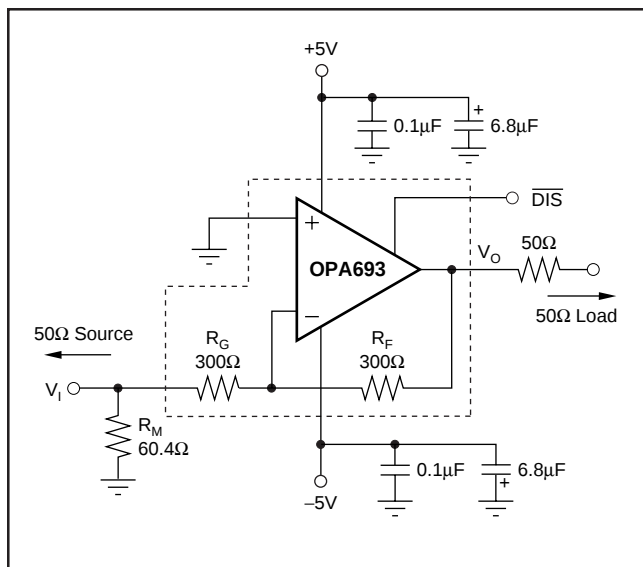
Figure 3. DC-Coupled, G = -1V/V , Bipolar-Supply Specification and Test Circuit.
