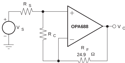
Figure 35. Unity-Gain Buffer
