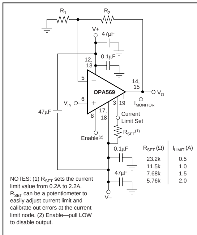
FIGURE 1. Basic Connections.
