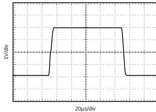
LARGE-SIGNAL STEP RESPONSE ( G = +1 , R_L = 10\Omega )
