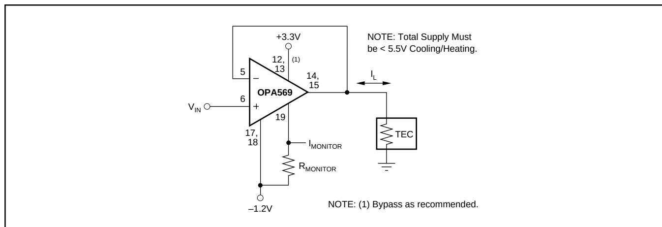
FIGURE 21. Single Power Amplifier Driving Bidirectional Current through a TEC using Asymmetrical Bipolar Power Supplies.
