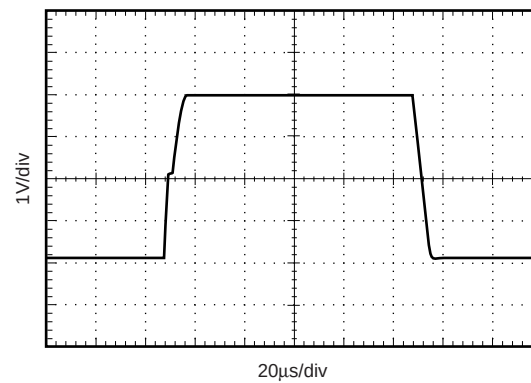
LARGE-SIGNAL STEP RESPONSE ( G = +1 , R_L = 1\Omega )
