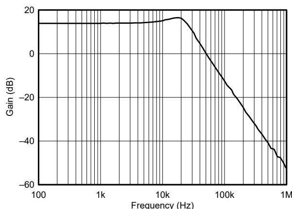
Figure 8-7. OPA4H014-SEP Second-Order, 25-kHz, Chebyshev, Low-Pass Filter
