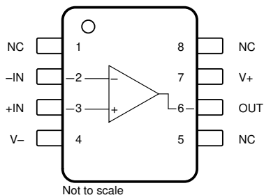
Figure 4-1. OPA486: D Package, 8-Pin SOIC (Top View)
