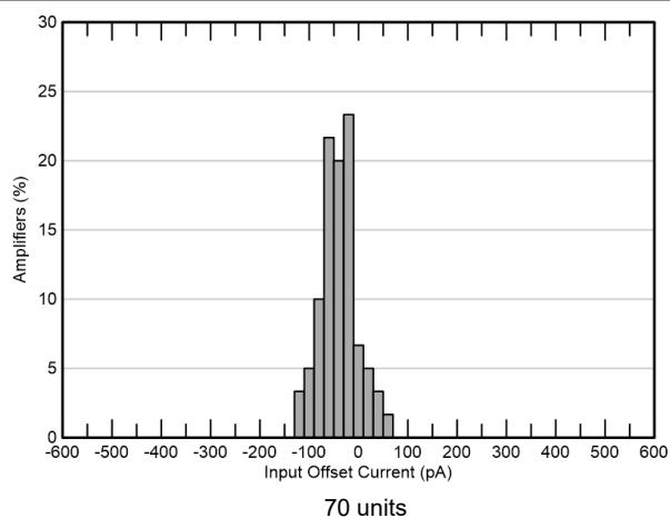
Figure 5-6. Input Offset Current Distribution
