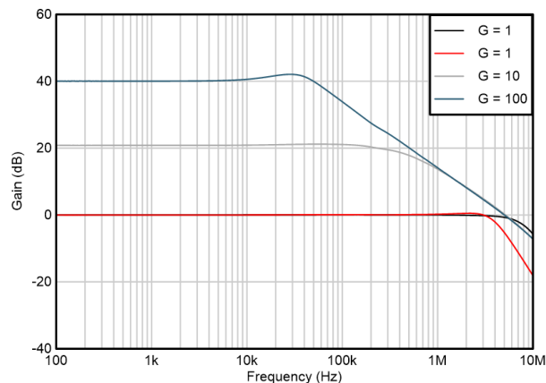
Figure 5-13. Closed-Loop Gain vs Frequency
