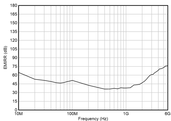
Figure 5-41. EMIRR vs Frequency
