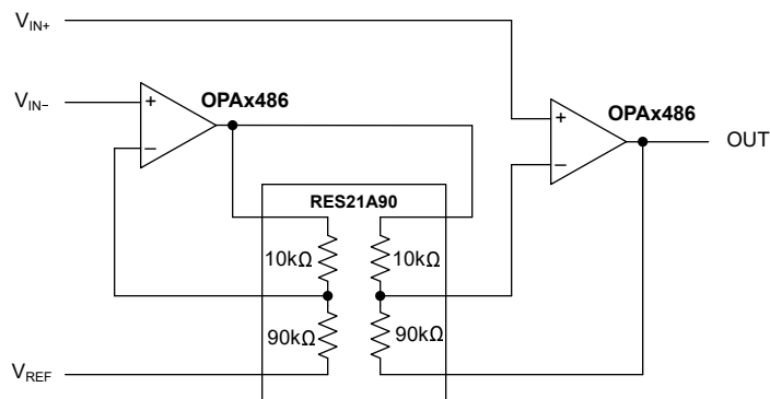
Figure 7-6. Two Op Amp Instrumentation Amplifier
