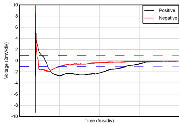
Figure 5-38. Settling Time
