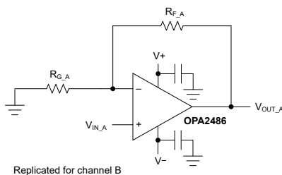
Figure 7-9. Schematic Representation
