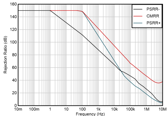
Figure 5-17. CMRR and PSRR vs Frequency
