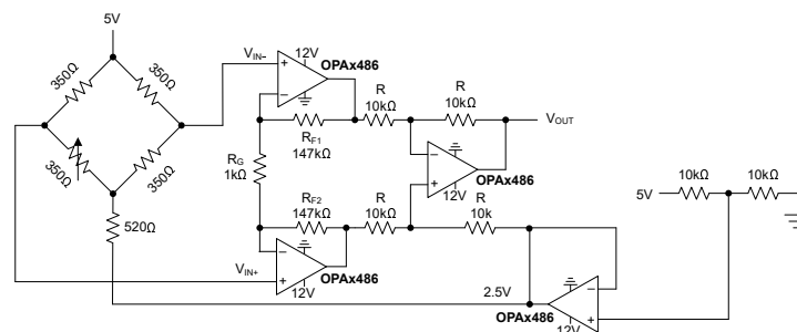
Instrumentation Amplifier
