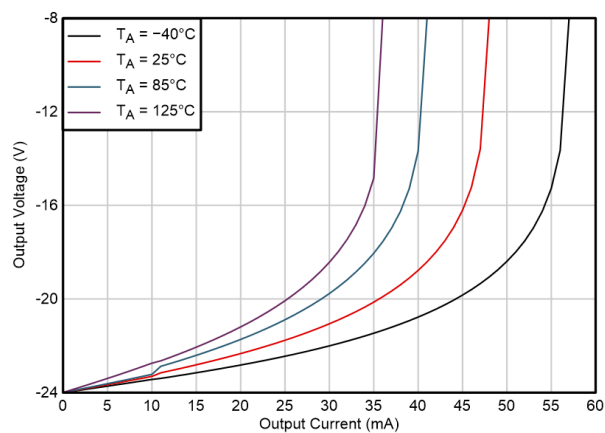
Figure 5-16. Output Voltage Swing vs Output Current (Sinking)
