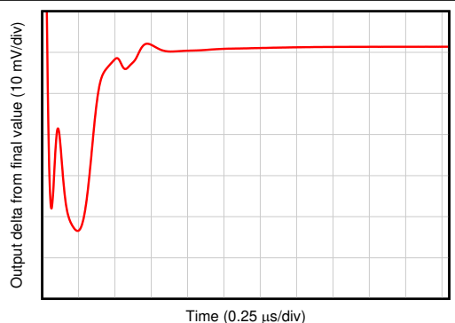
Figure 6-45. Small-Signal Step Response
