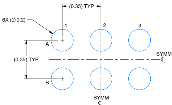
LAND PATTERN EXAMPLE EXPOSED METAL SHOWN SCALE: 60X
