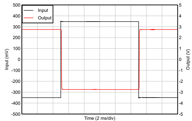
Figure 5-30. Overload Recovery
