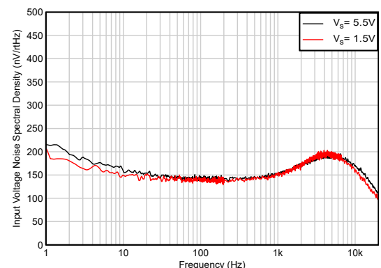
Figure 5-24. Input Voltage Noise Spectral Density
