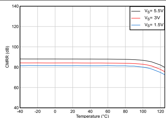
Figure 5-22. DC CMRR vs Temp ( V_- \geq V_{CM} \geq (V_+) - 0.7\text{V} )
