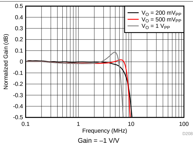
Figure 20. Inverting Large-Signal Frequency Response Flatness
