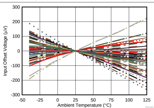
32 units at 5-V and 3-V supply, Input offset voltage calibrated to 0V at 25°C
