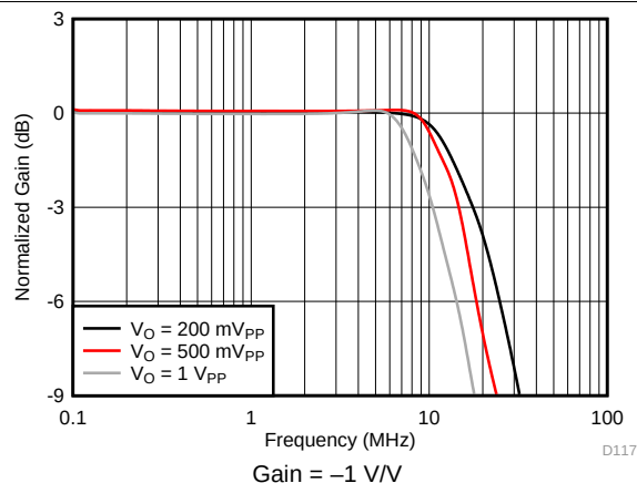
Figure 18. Inverting Large-Signal Bandwidth
