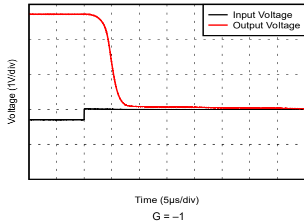
Figure 5-34. Overload Recovery
