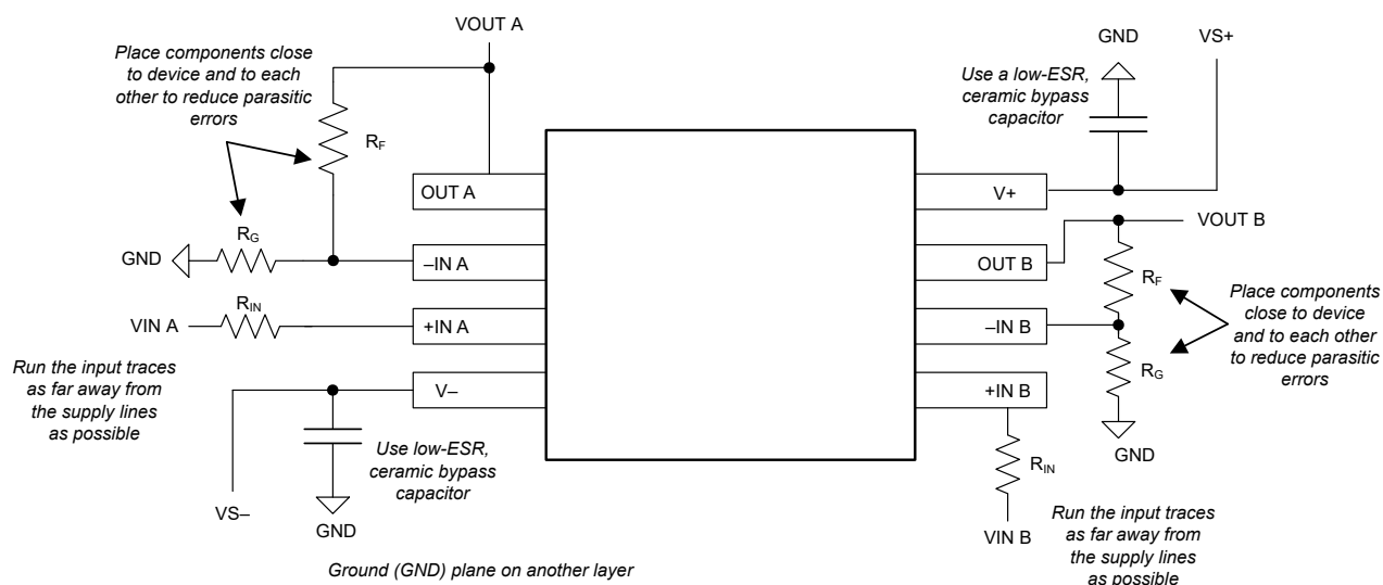
Figure 7-5. Layout Example
