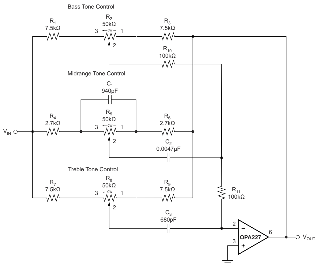
Figure 8-12. Three-Band Active Tone Control (Bass, Midrange, and Treble)
