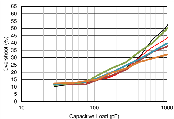
Figure 7-26. Small-Signal Overshoot vs Capacitive Load 10-mV Step
