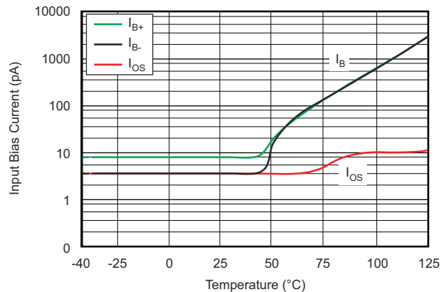
Figure 5-8. Input Bias Current vs Temperature
