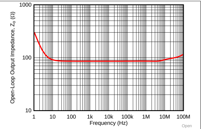
Figure 20. Open-Loop Output Impedance vs Frequency
