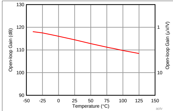
Figure 19. Open-Loop Gain vs Temperature
