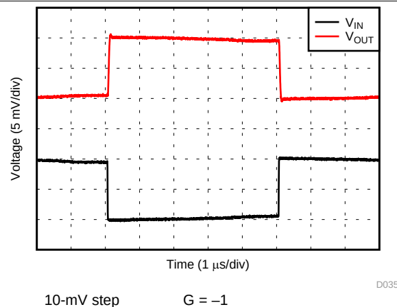
Figure 26. Small-Signal Step Response
