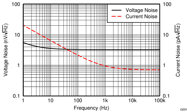
Figure 5-1. Input Voltage Noise Density and Input Current Noise Density vs Frequency
