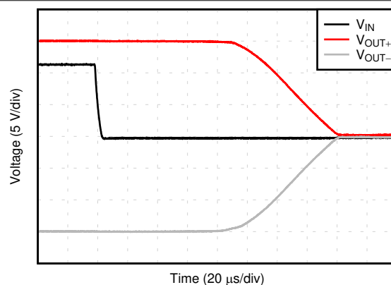
Figure 6-38. Power-Down Time (PD High to Low)
