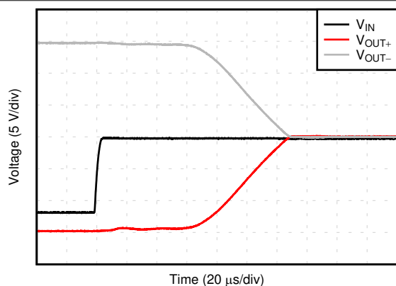
Figure 6-37. Power-Down Time (PD Low to High)
