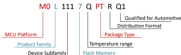
Figure 10-1. Device Nomenclature
