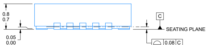
SECTION A-A TYPICAL
