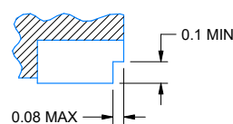
SECTION A-A TYPICAL
