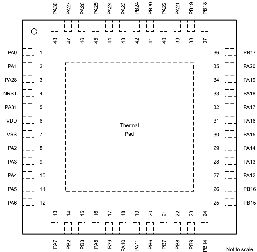
Figure 6-2. 48-Pin RGZ (VQFN) (Top View)
