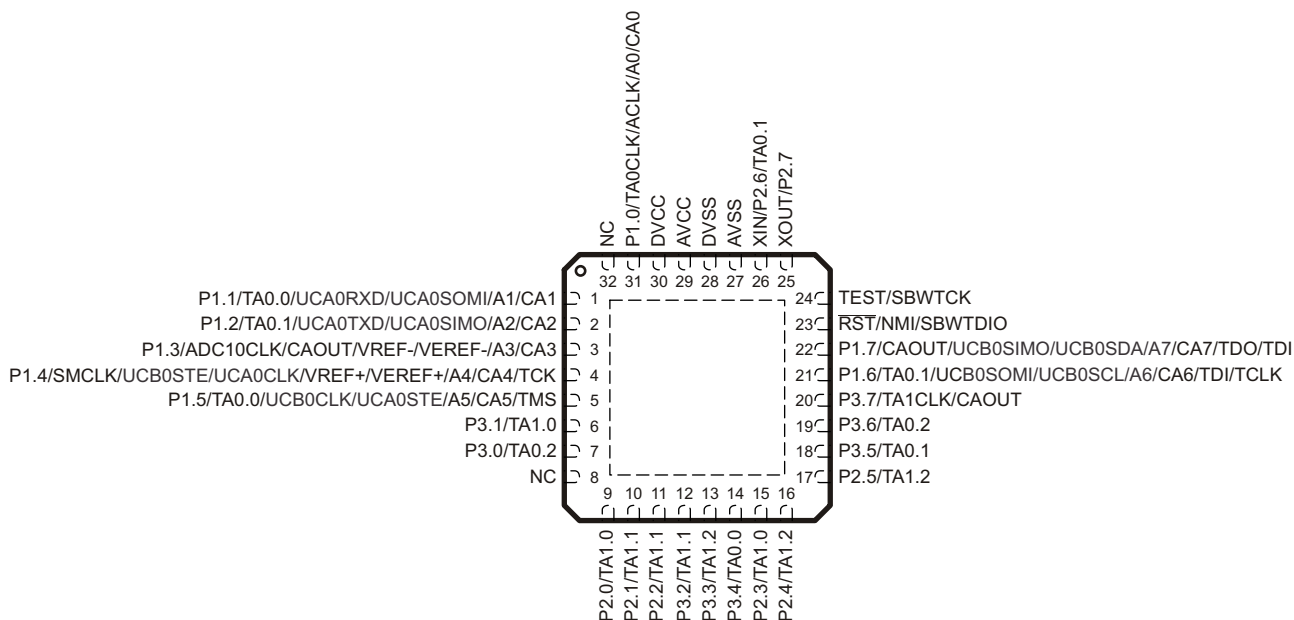
RHB32 PACKAGE (TOP VIEW)
