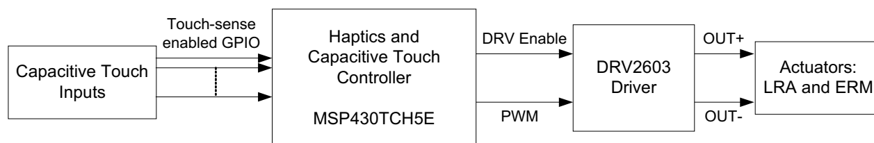
Figure 1. Stand-Alone Application With MSP430TCH5E Device as Haptics and Capacitive Touch Controller
