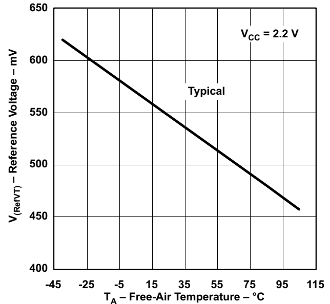
Figure 25. V (RefVT) vs Temperature, V CC = 2.2 V
