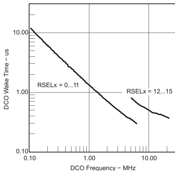
Figure 16. DCO Wake-Up Time From LPM3 vs DCO Frequency
