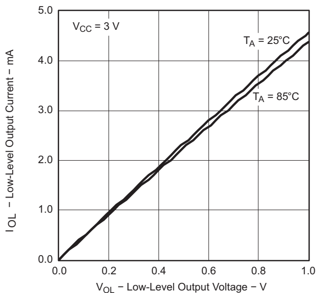
Figure 18. USI Low-Level Output Voltage vs Output Current
