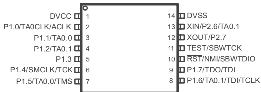
N or PW PACKAGE (TOP VIEW)
