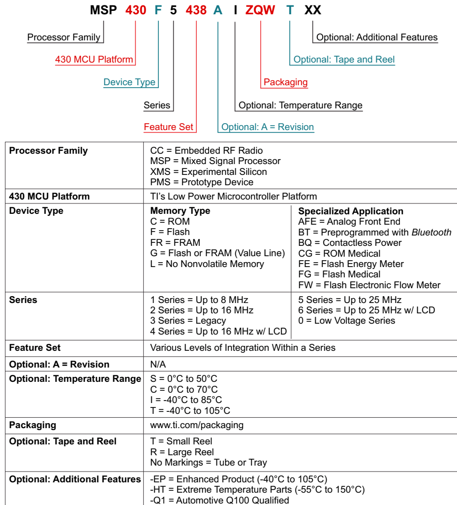
Figure 8-1. Device Nomenclature
