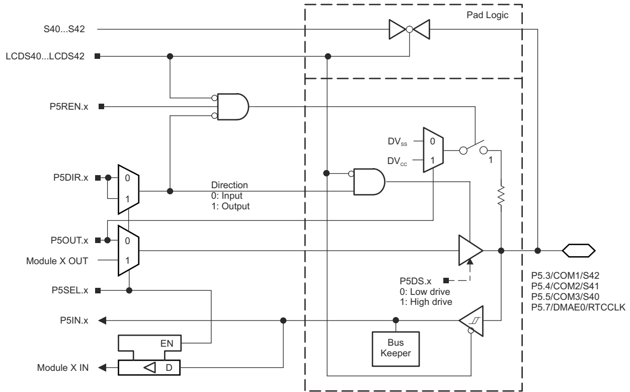
Figure 9-9. Port P5 (P5.3 to P5.5 and P5.7) Diagram
