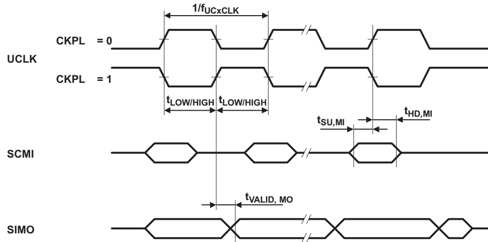
Figure 4-29. SPI Master Mode, CKPH = 1
