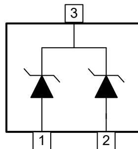
Functional Diagram
