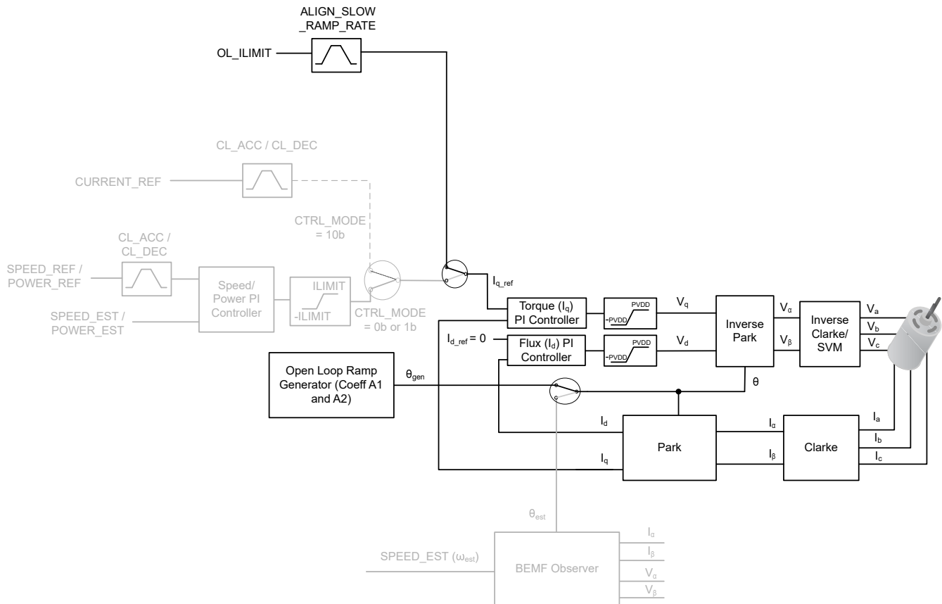
Figure 7-27. Open Loop
