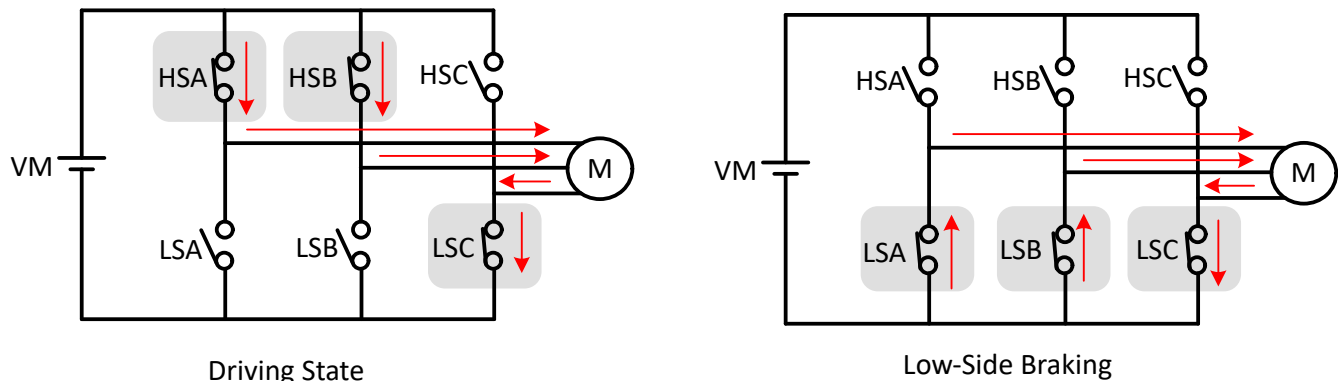
Figure 7-45. Low-Side Braking
