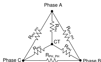
Figure 7-38. Motor Resistance
