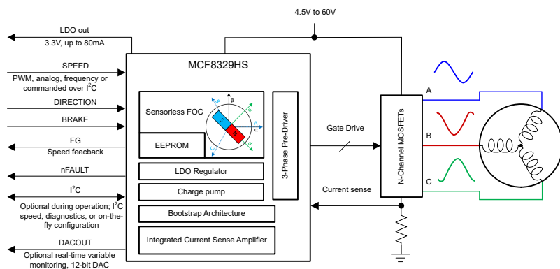
Simplified Schematic
