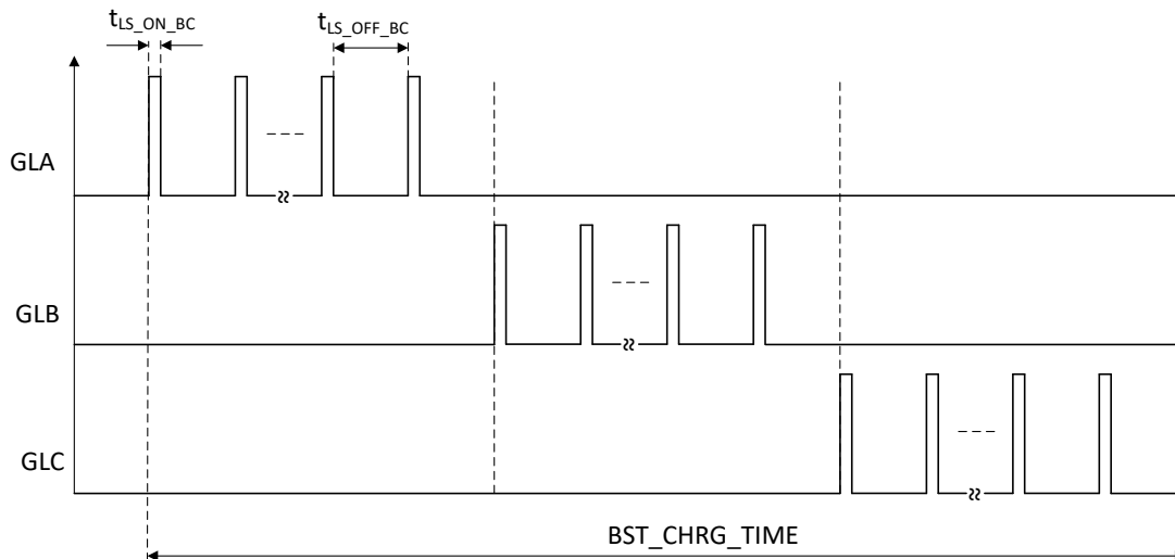
Figure 7-20. Bootstrap Capacitor Precharging at Start-up
