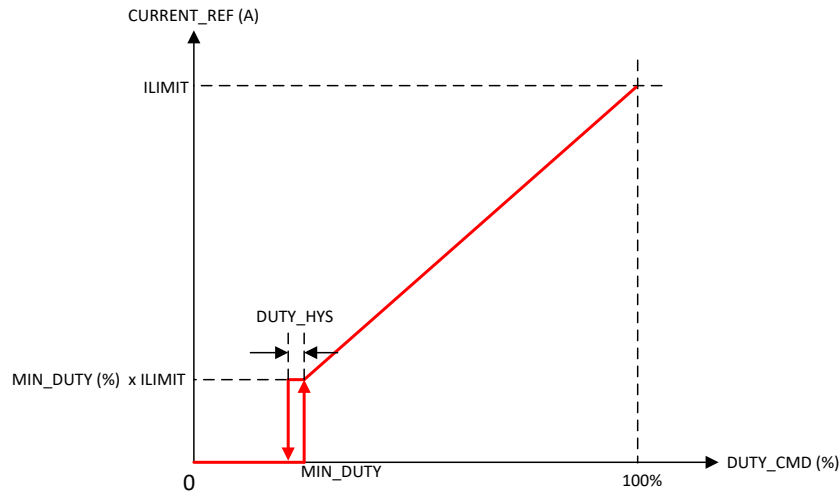
Figure 7-19. Current Reference Transfer Function
