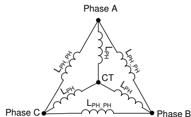
Figure 7-39. Motor Inductance
