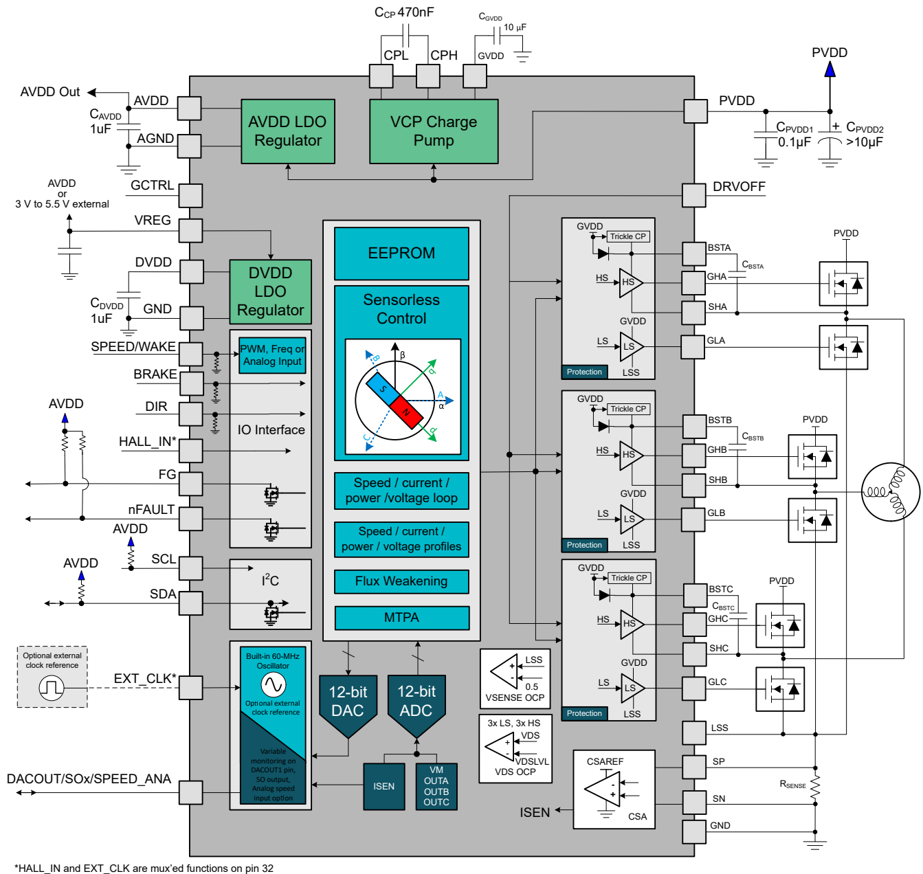
Figure 7-1. MCF8329HS Functional Block Diagram
