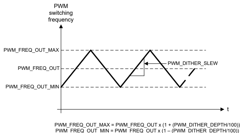
Figure 7-43. Triangular PWM Dithering
