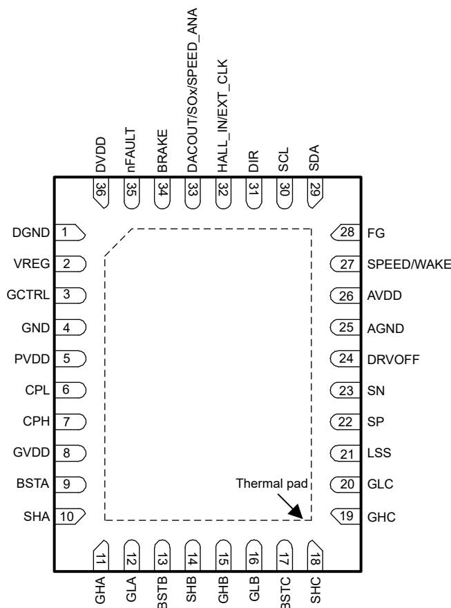
Figure 5-1. MCF8329HS36-Pin WQFN With Exposed Thermal PadTop View
