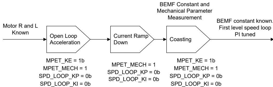
Figure 7-41. MPET Sequence
