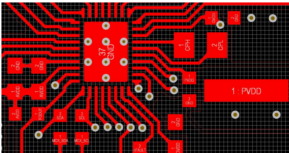
Figure 10-7. Layout example of MCF8329HS device
