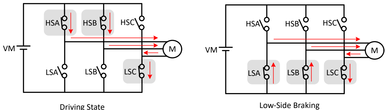
Figure 6-44. Low-Side Braking
