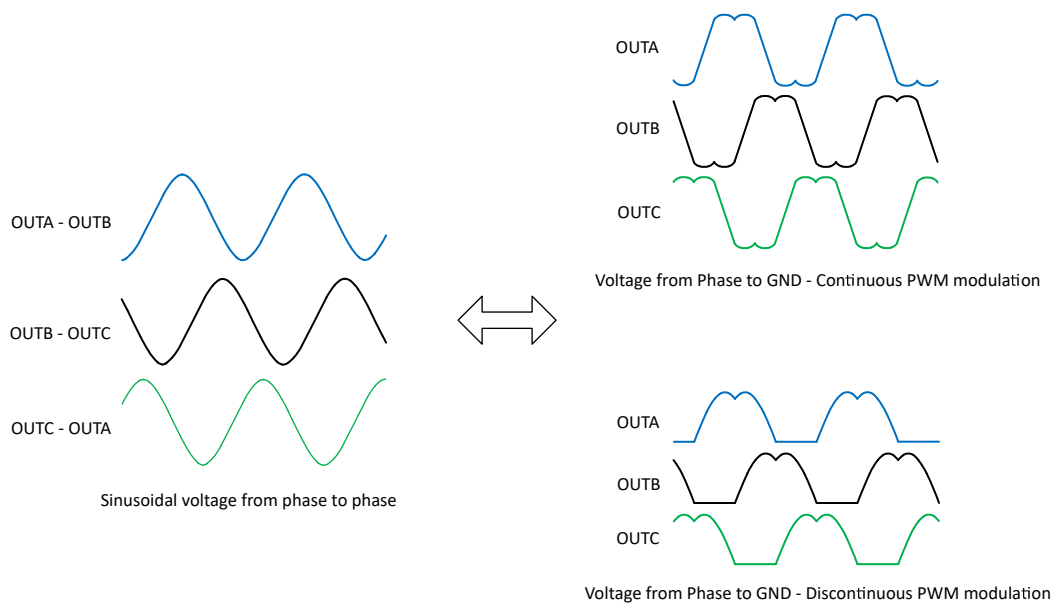
Figure 6-42. Continuous and Discontinuous PWM Modulation Phase Voltages
