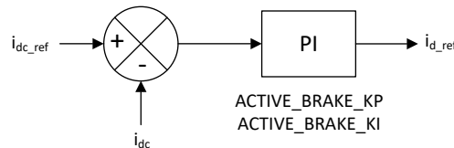
Figure 6-41. Active Braking Current Control Loop for i_{d\_ref}
