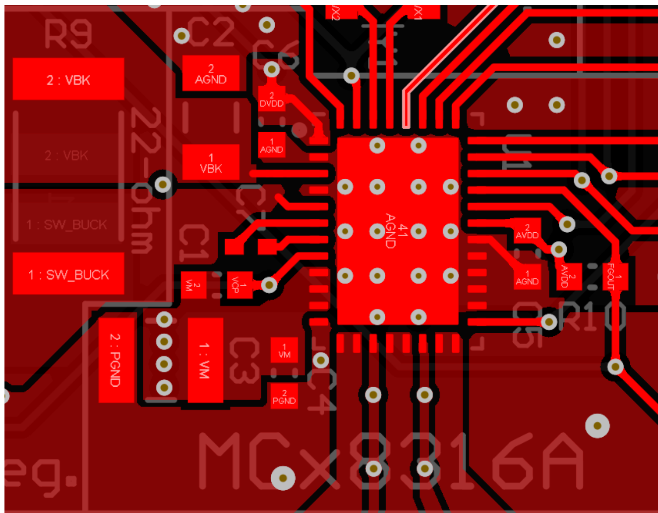
Figure 9-12. Recommended Layout Example
