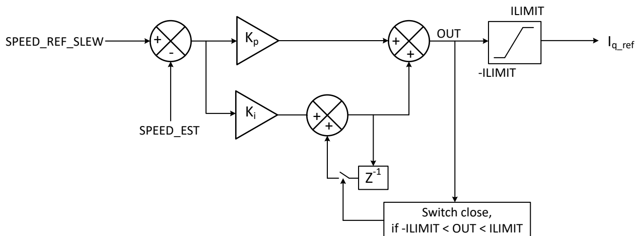
Figure 6-34. Speed PI Control
