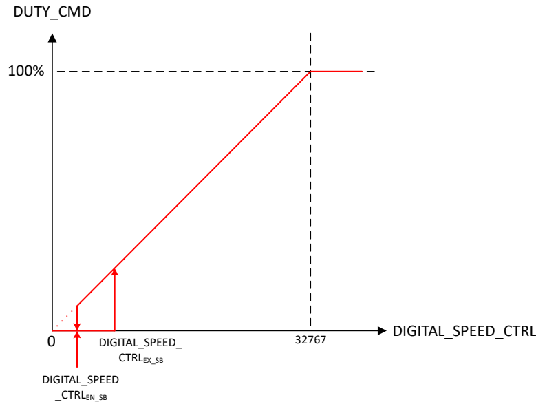
Figure 6-16. I 2 C-Mode Motor Control
