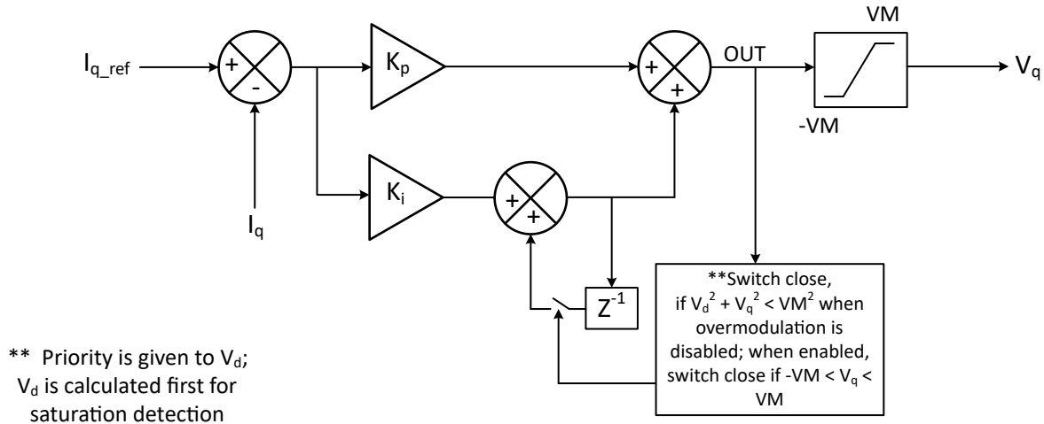
Figure 6-36. I_q Current PI Control
