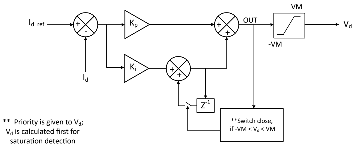
Figure 6-35. I_d Current PI Control
