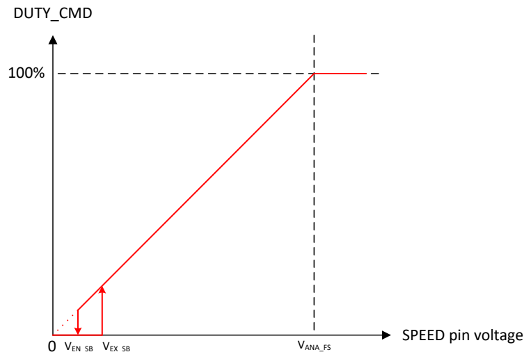
Figure 6-14. Analog-Mode Motor Control
