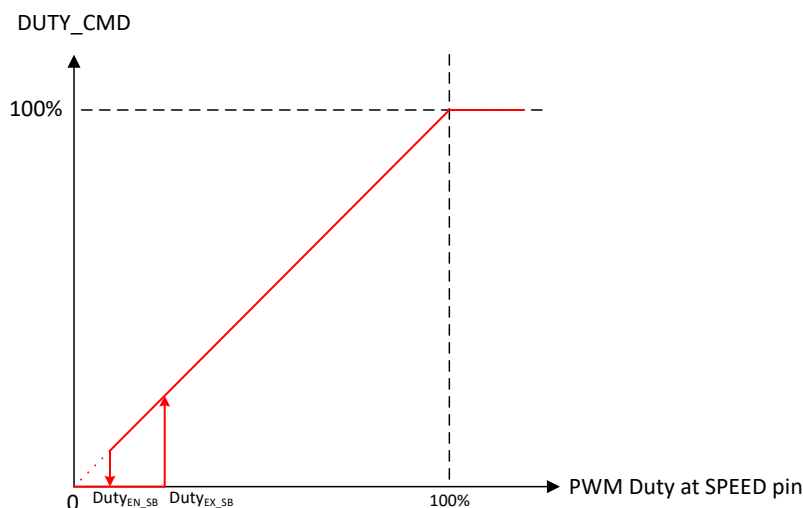
Figure 6-15. PWM-Mode Motor Control
