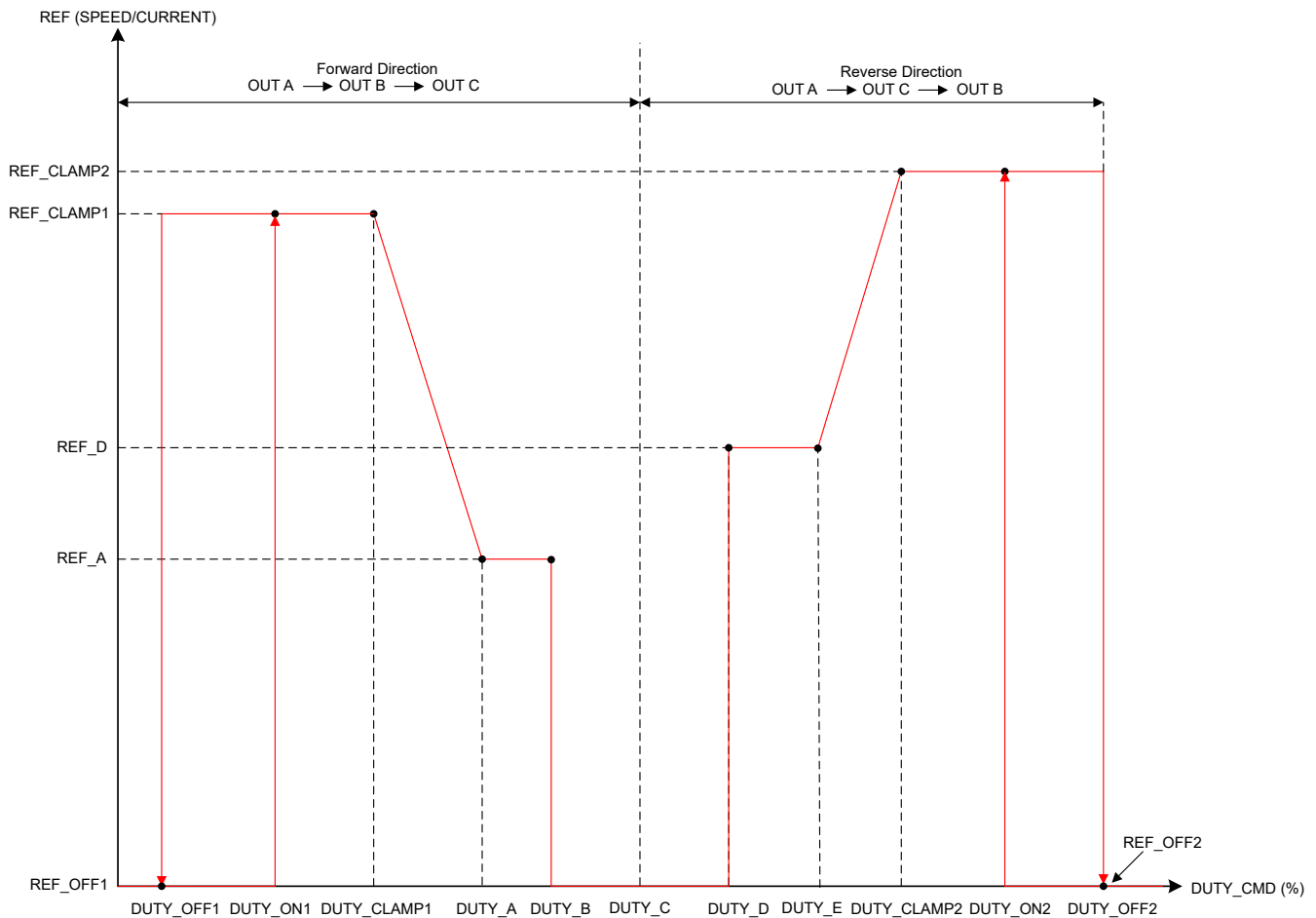
Figure 6-20. Forward-Reverse Reference Profile
