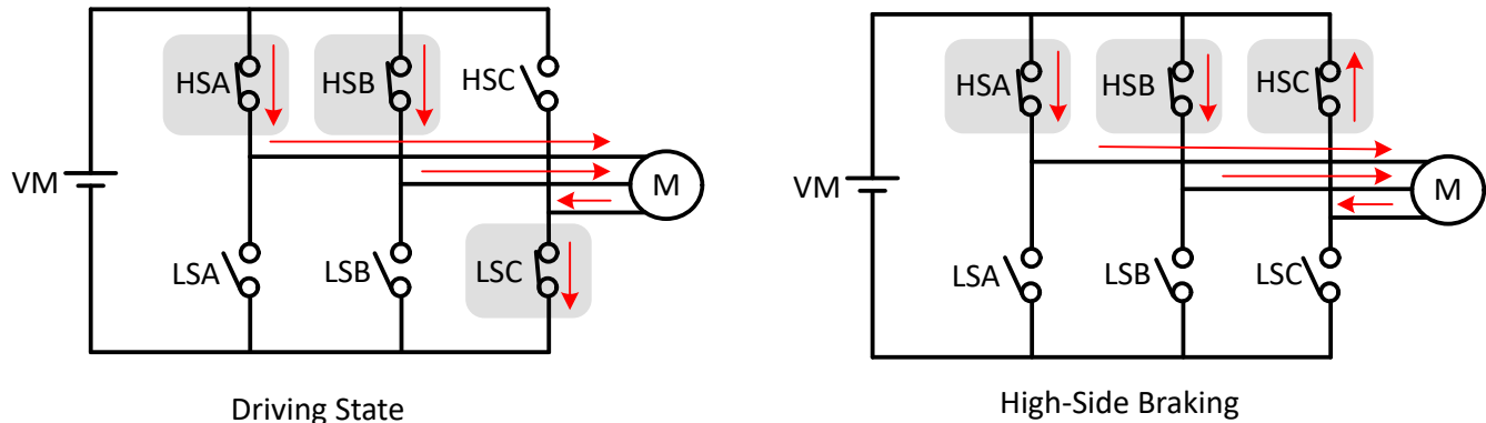
Figure 6-45. High-Side Braking
