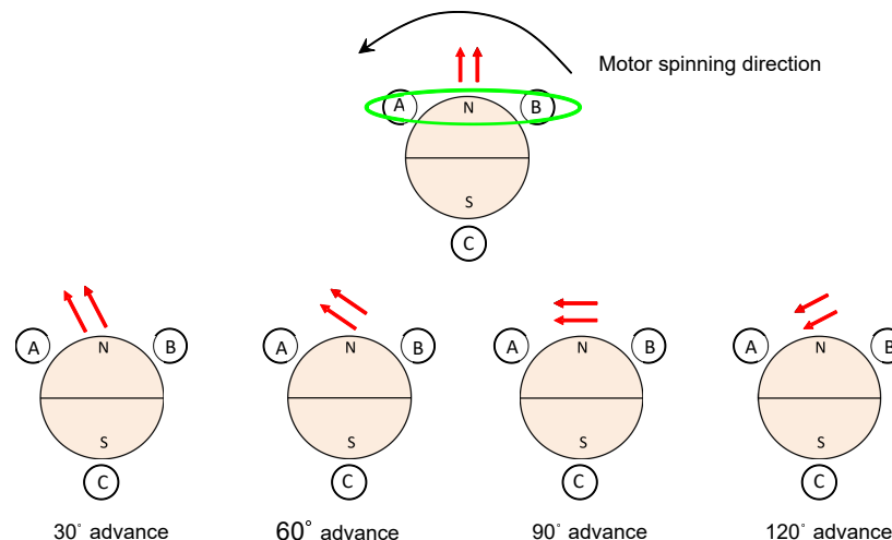
Figure 6-28. IPD Advance Angle
