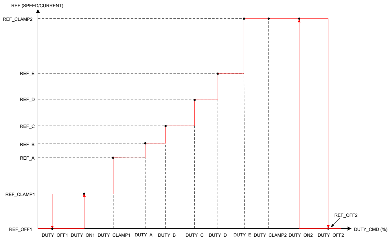
Figure 6-19. Staircase Reference Profile
