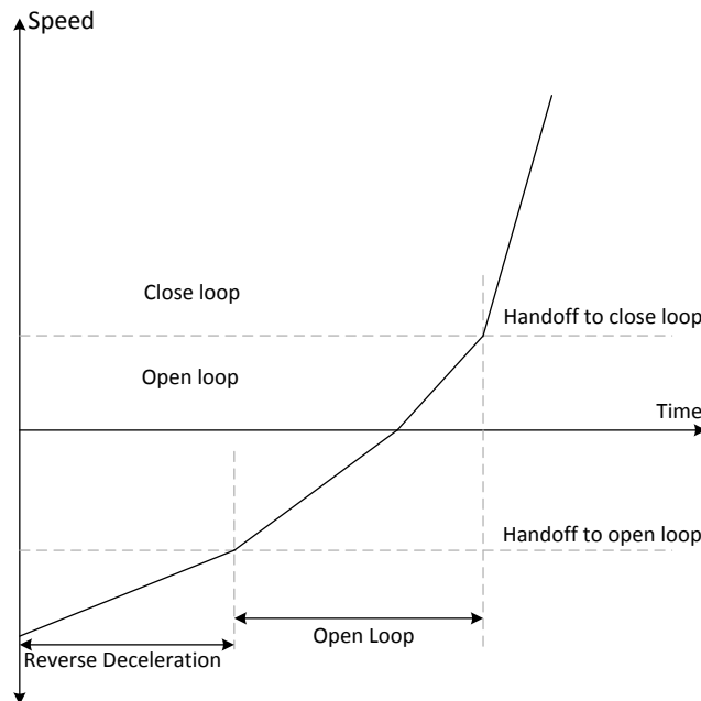
Figure 6-24. Reverse Drive Function
