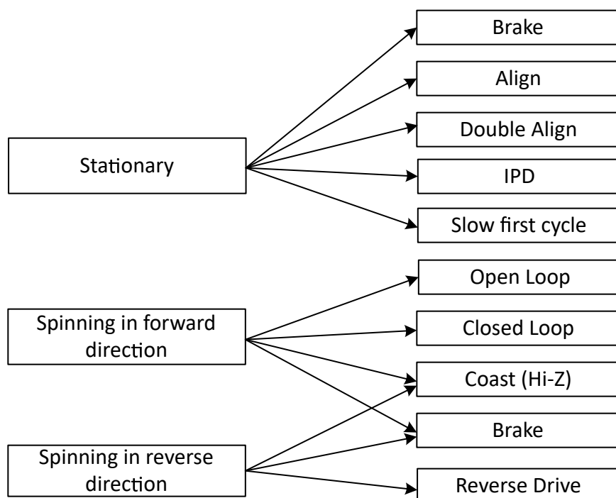
Figure 6-21. Starting the motor under different initial conditions
