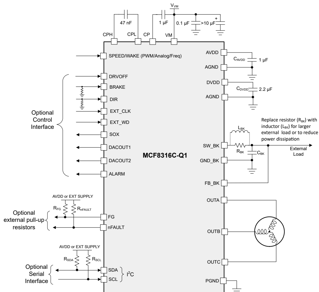
Figure 9-1. Example Application Schematic
