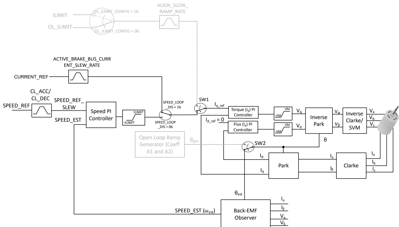
Figure 6-31. Open to Closed Loop Transition Control Block Diagram
