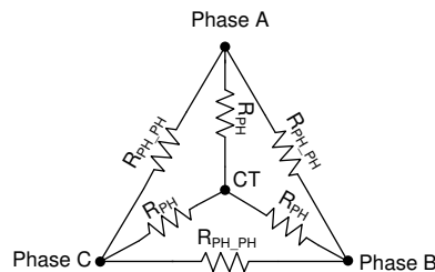
Figure 6-37. Motor Resistance
