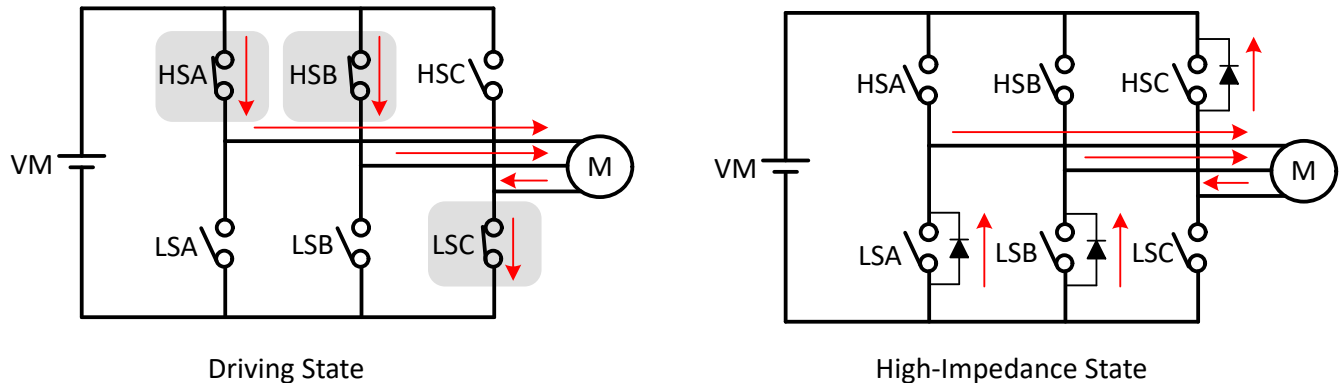
Figure 6-43. Coast (Hi-Z) Mode
