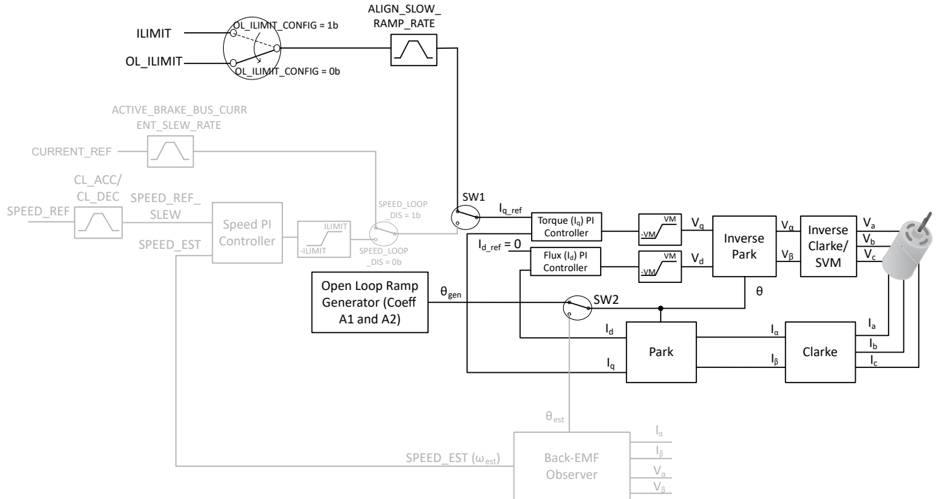
Figure 6-29. Open Loop
