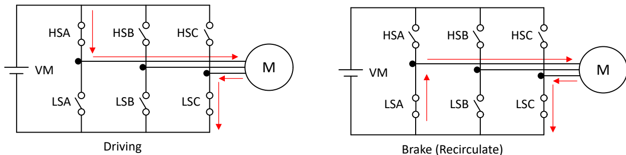
Figure 6-26. IPD Release Mode - Brake (0b)
