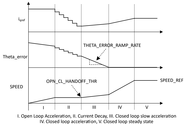
Figure 6-30. Control Sequence in Open to Closed Loop Transition
