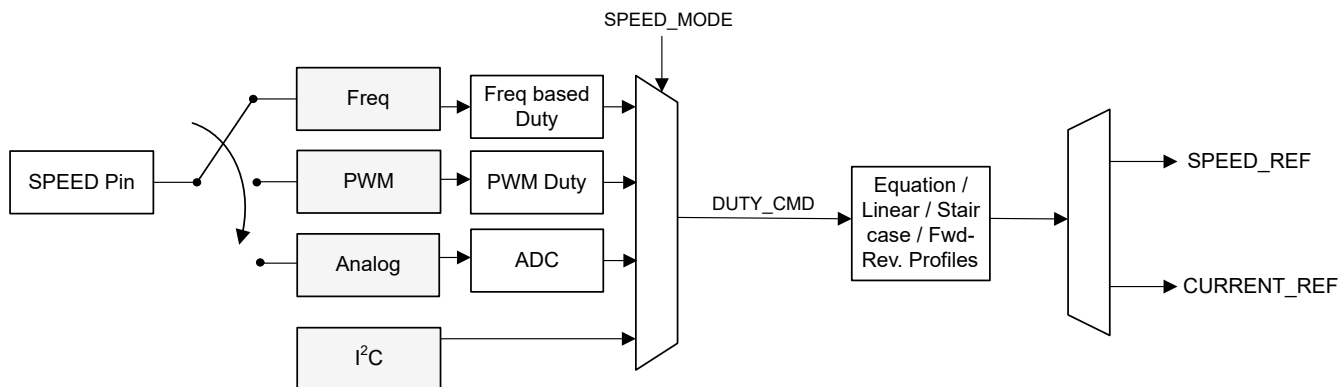
Figure 6-13. Multiplexing the Input Reference Source
