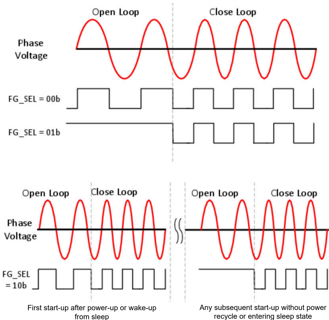
Figure 6-47. FG Behavior During Open Loop
