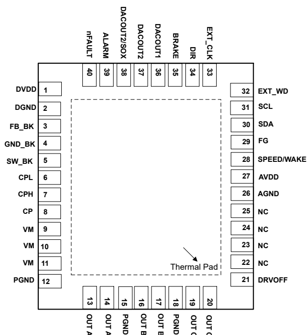
Figure 4-1. MCF8316C-Q1, 40-Pin VQFN With Exposed Thermal Pad, Top View
