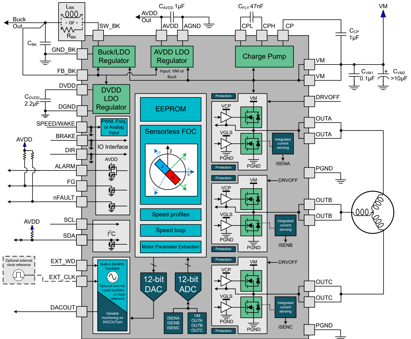
Figure 6-1. MCF8316C-Q1 Functional Block Diagram
