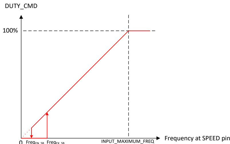
Figure 6-17. Frequency-Mode Motor Control
