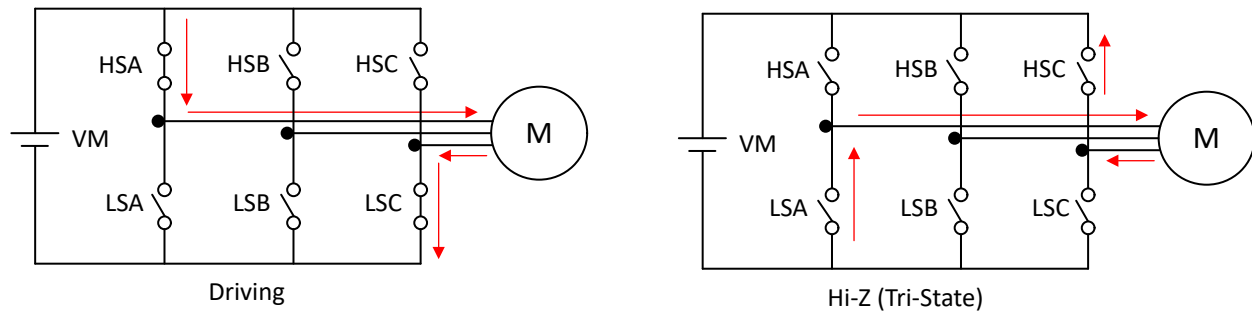
Figure 6-27. IPD Release Mode - Tristate (1b)
