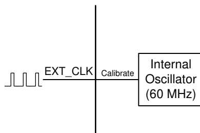
Figure 6-66. External Clock Reference
