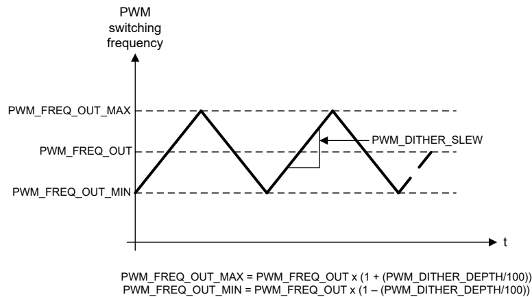
Figure 6-53. Triangular PWM Dithering
