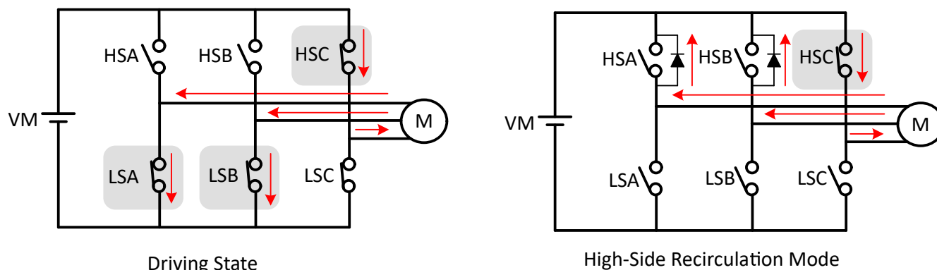
Figure 6-57. High-Side Recirculation
