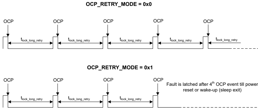
Figure 6-26. OCP retry Modes
