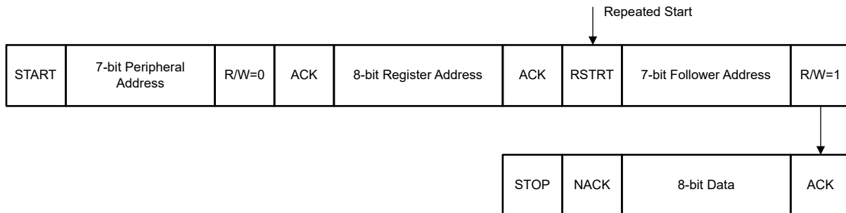
Figure 6-30. I²C Read Sequence
