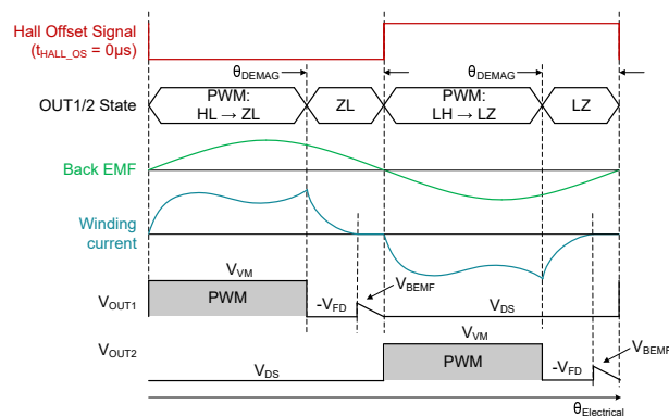
Figure 6-16. Detailed Timing Diagram for Square Commutation Using Asynchronous Mode for \theta_{\text{DEMAG}}
