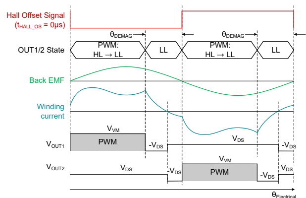
Figure 6-17. Detailed Timing Diagram for Square Commutation Using Synchronous Mode for \theta_{\text{DEMAG}}
