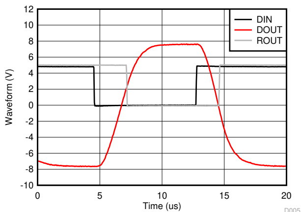
Figure 7-2. Loopback Waveforms
