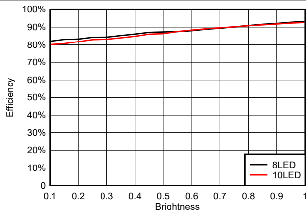
Figure 6-8. Efficiency at 0.5A Max Output Current, 22uH Inductor, Boost Topology
