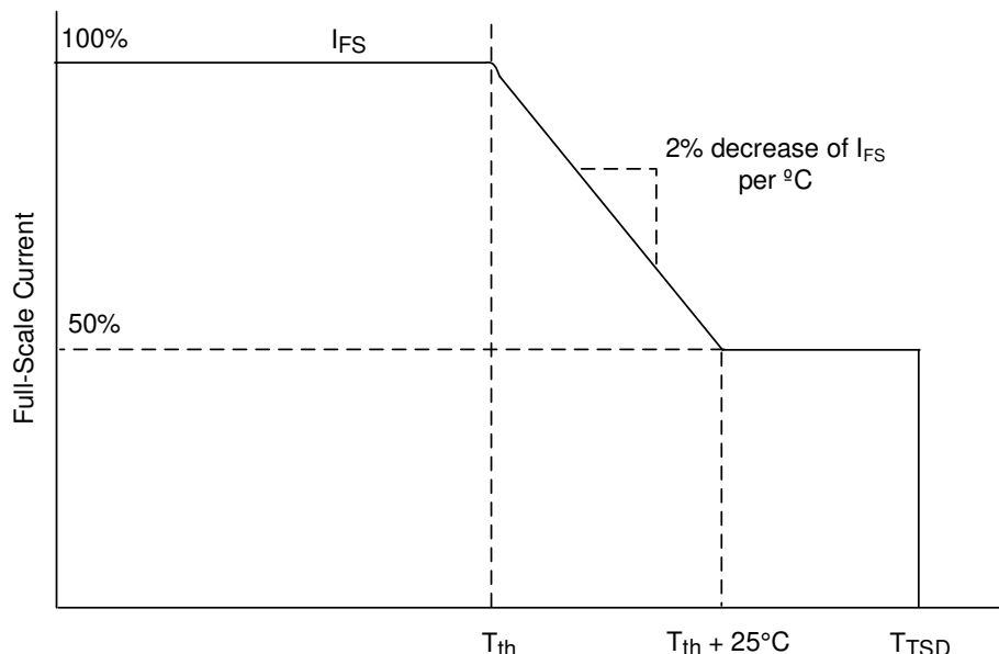
Figure 7-4. Thermal Foldback
