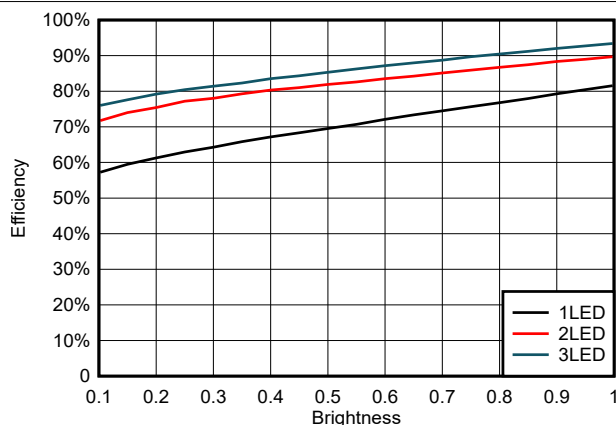
Figure 6-10. Efficiency at 1.5A Max Output Current, 22uH Inductor, Buck Topology
