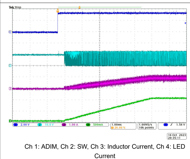
Figure 8-19. Startup at ADIM = 100%, 500Hz
