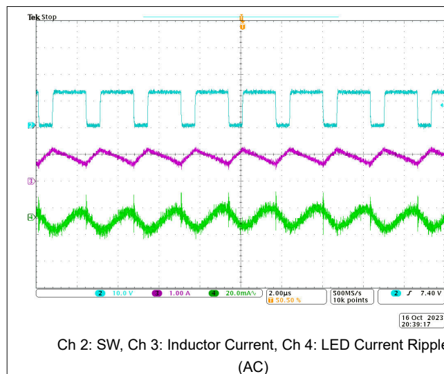
Figure 8-16. LED Current Ripple at ADIM = 100%, 1kHz and F_{SW} = 400\text{kHz}
