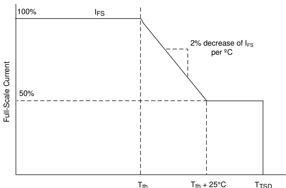
Figure 7-4. Thermal Foldback
