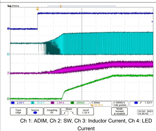
Figure 8-5. Startup at ADIM = 100%, 500Hz
