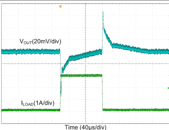
Figure 8-15. Buck Transient from PFM-to-PWM Mode
