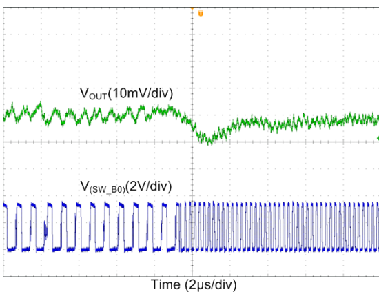
Figure 8-13. Buck Output Voltage Ripple, Forced-PWM Mode
