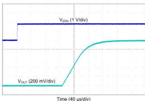
Figure 8-24. LDO Start-Up
