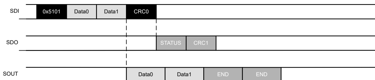
Figure 7-12. Example of FWD_WR_END command
