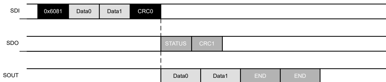
Figure 7-13. Example of FWD_RD_END_CRC command
