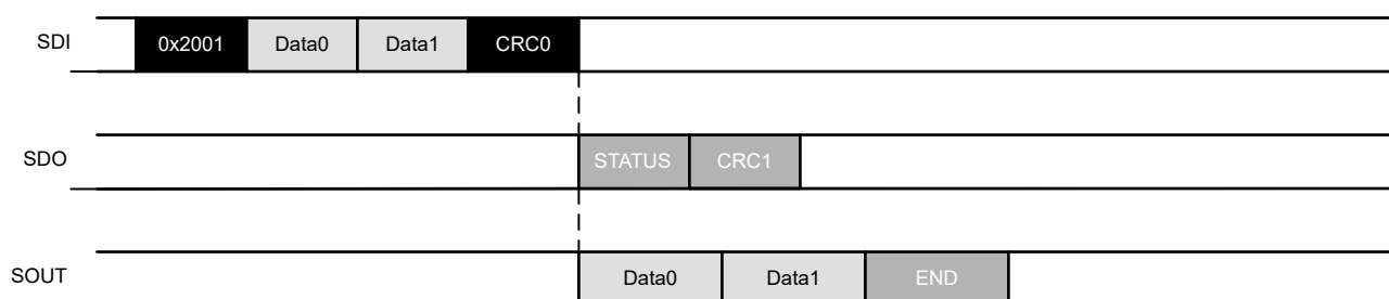
Figure 7-9. Example of FWD_WR_CRC command
