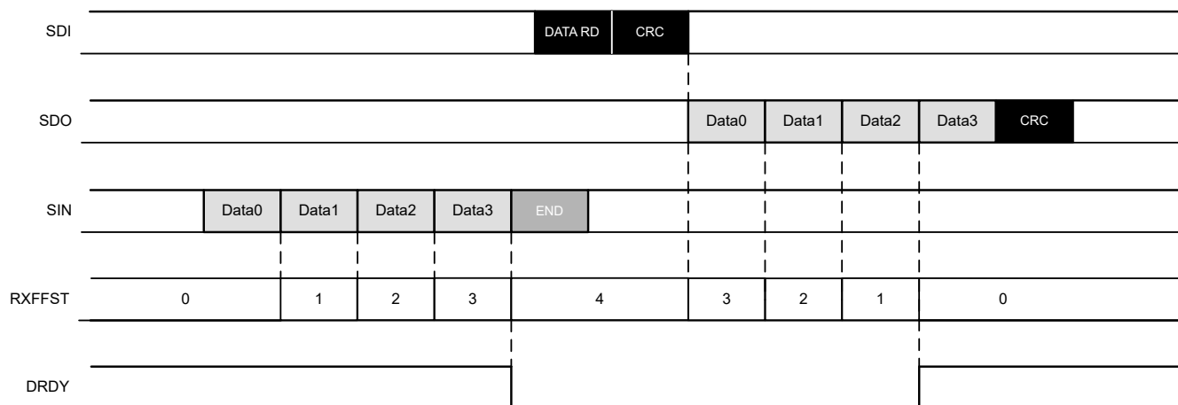
Figure 7-6. Example of DRDY pin with RXFFLVL register set to 3
