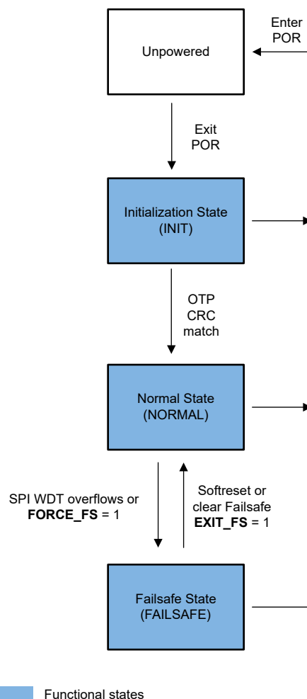
Figure 7-7. Device Functional Modes
