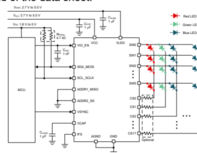
Simplified Schematic
