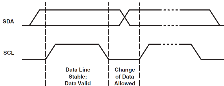
Figure 7-8. Data Validity
