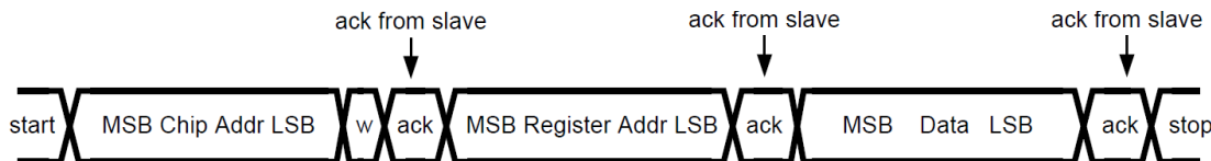
Figure 7-11. Write Cycle
