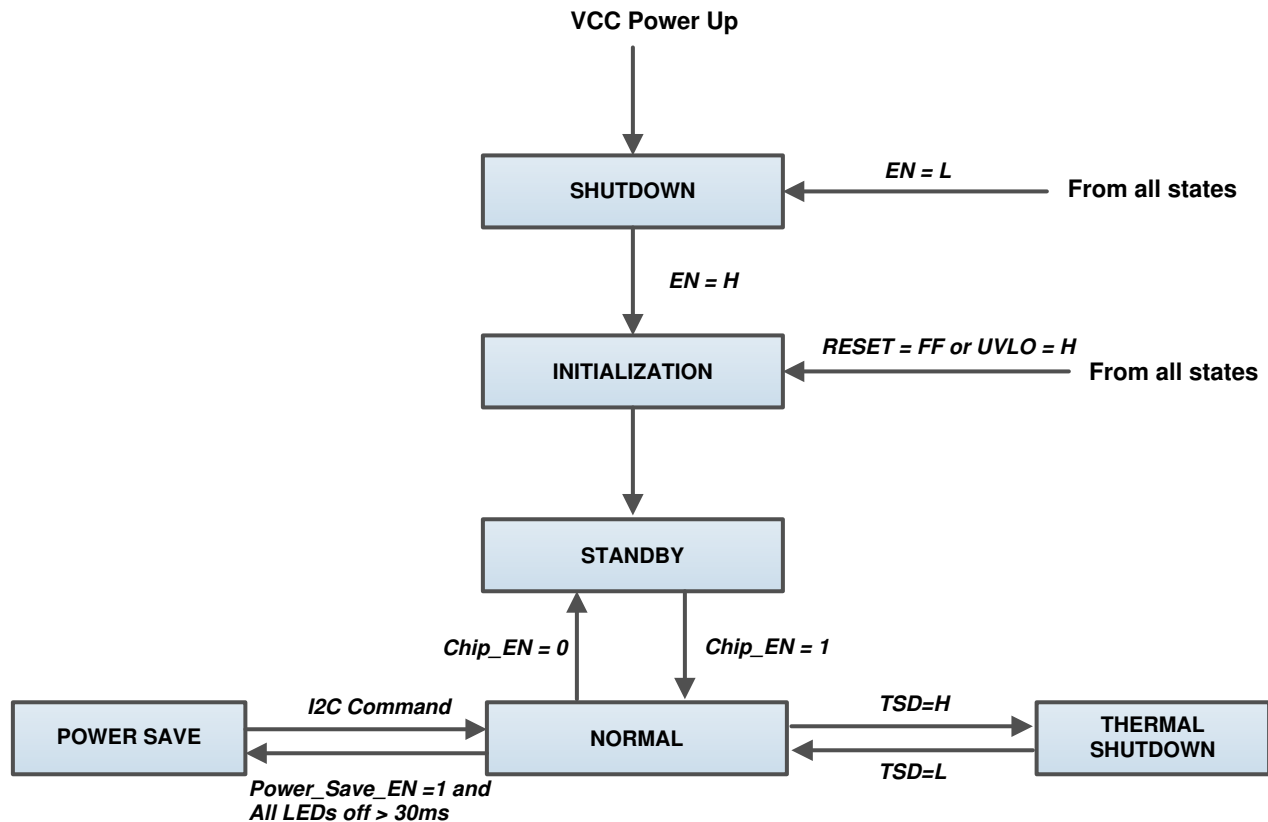
Figure 7-7. Functional Modes
