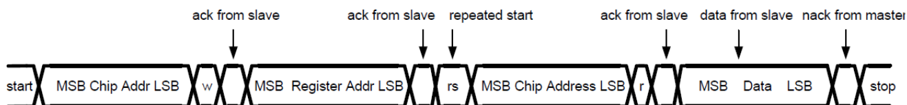
Figure 7-12. Read Cycle
