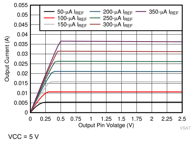
Figure 6-8. OUT Pin Voltage vs Output Current
