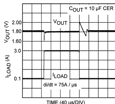
Figure 16. Load Transient Response: 10-μF Ceramic, 75 A/μs di/dt
