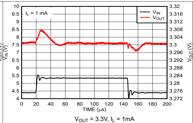
Figure 5-14. Line Transient Response (New Chip)
