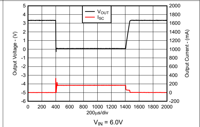
Figure 5-16. Short-Circuit Current vs Time (New Chip)
