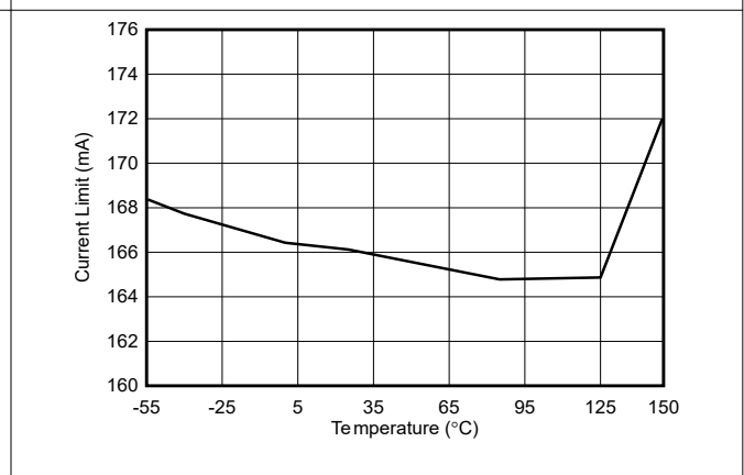
Figure 5-18. Instantaneous Short-Circuit Current vs Temperature (New Chip)
