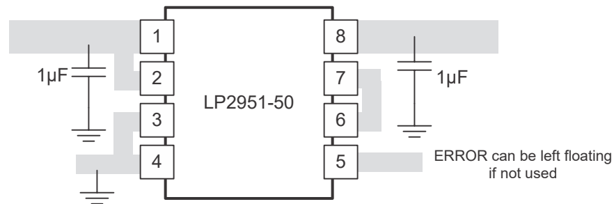
Figure 7-7. LP2951 Layout Example (D or P Package)
