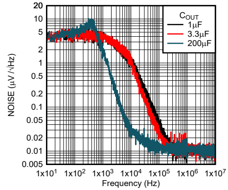
Figure 5-62. Output Noise vs Frequency (New Chip)
