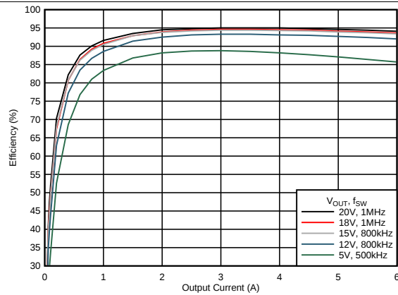
Figure 21. Efficiency vs Output Current
