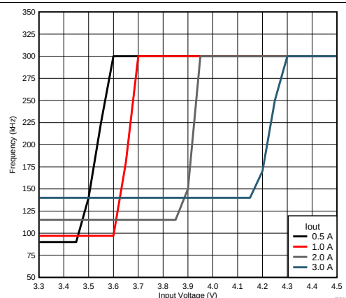
Figure 21. Frequency Foldback
