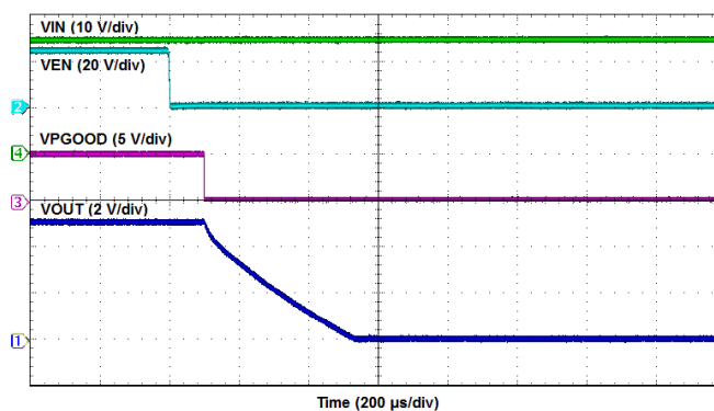
Figure 30. Enable Turn-OFF
