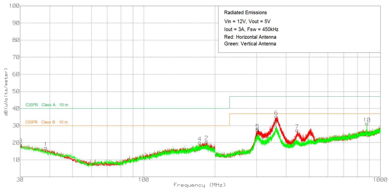
Figure 45. Radiated Emissions 12-V Input, 5-V Output, 3-A Load (EN55011 Class B)
