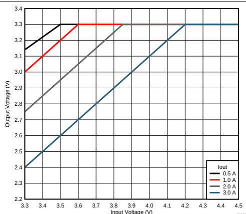
Figure 20. Voltage Dropout
