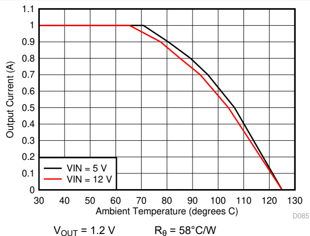
Figure 6-17. Ambient Temperature vs Output Current
