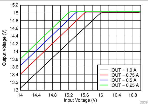
Figure 6-4. Dropout Voltage
