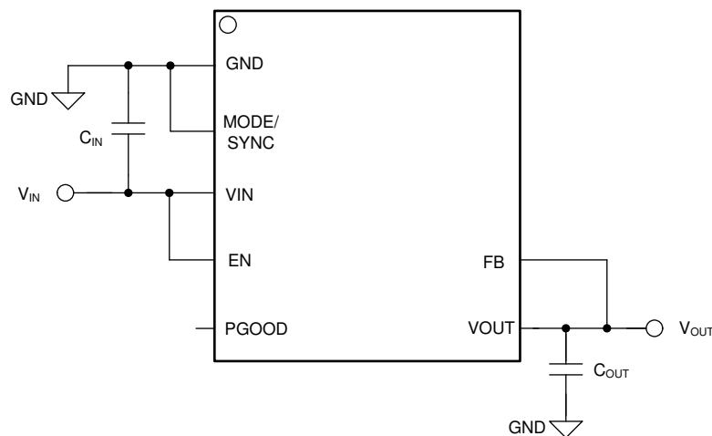
Figure 8-1. Fixed 5-V or 3.3-V Typical Application Circuit
