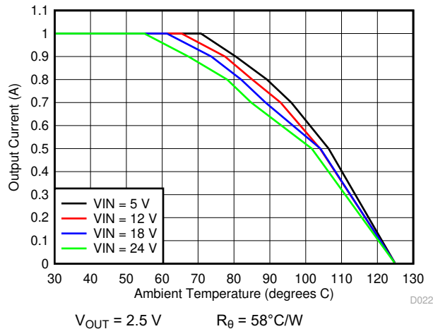
Figure 6-19. Ambient Temperature vs Output Current
