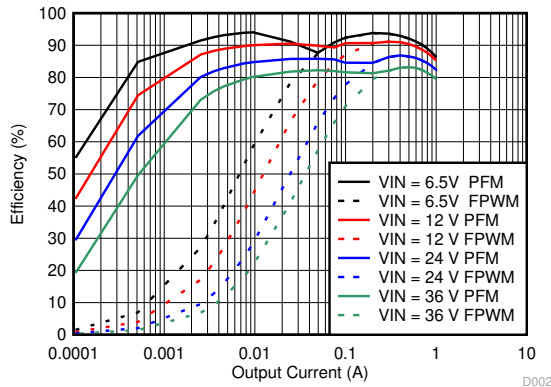
Figure 8-6. Efficiency
