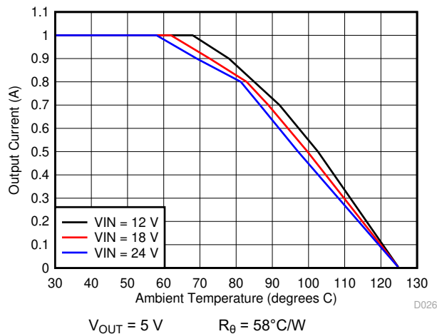
Figure 6-21. Ambient Temperature vs Output Current
