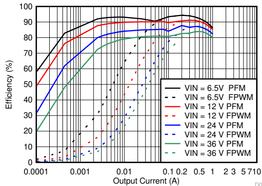
Figure 8-42. Efficiency for V_{OUT} = 5\text{ V}
