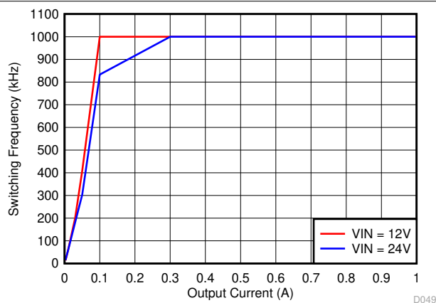
Figure 6-27. Auto PFM Mode Switching Frequency vs Output Current
