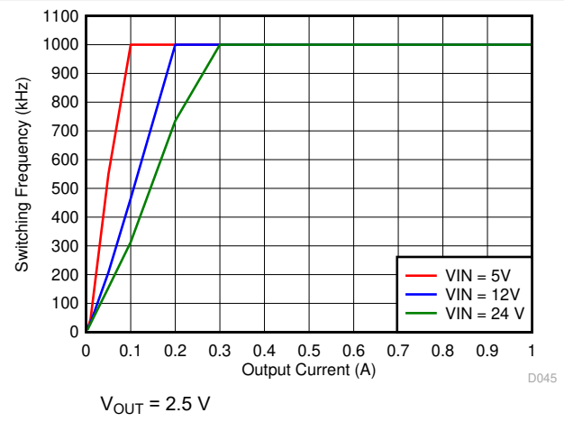
Figure 6-24. Auto PFM Mode Switching Frequency vs Output Current
