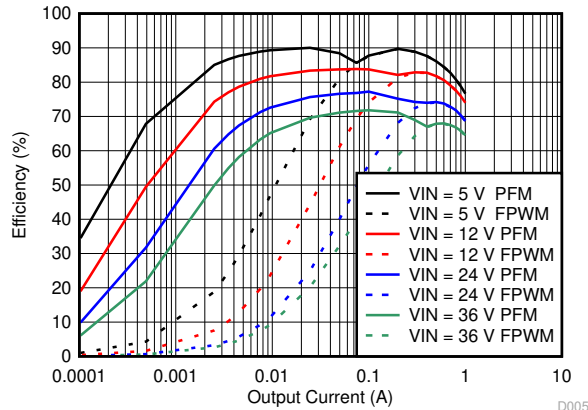
Figure 8-30. Efficiency
