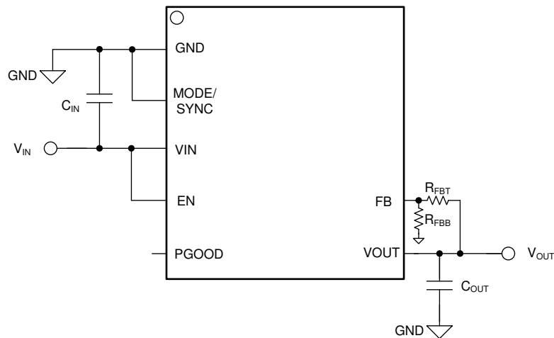
Figure 8-4. Adjustable 1.2-V to 15-V Output Typical Application Circuit
