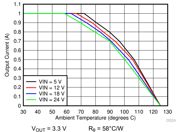
Figure 6-20. Ambient Temperature vs Output Current
