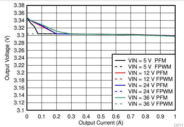
Figure 8-45. Line and Load Regulation for V_{OUT} = 3.3\text{ V}
