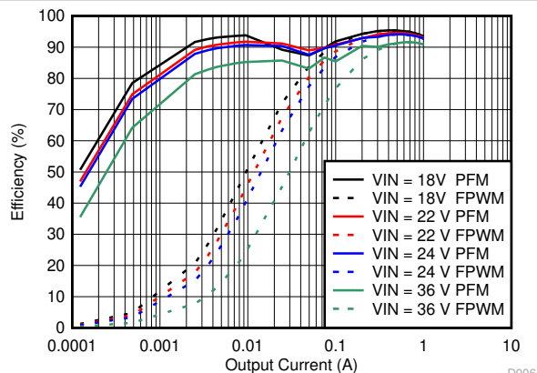
Figure 8-24. Efficiency
