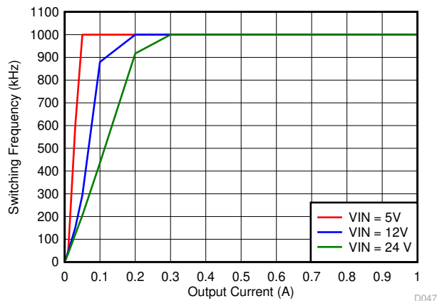
Figure 6-25. Auto PFM Mode Switching Frequency vs Output Current
