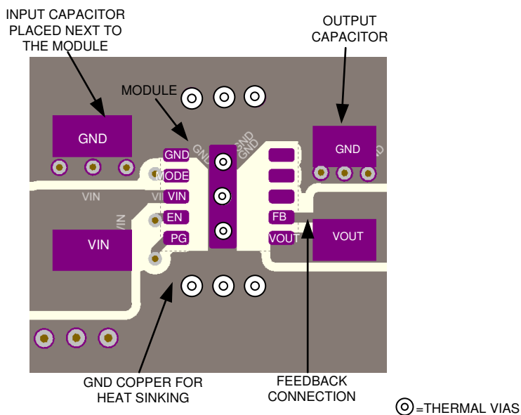
Figure 8-49. Layout Example With Fixed Output Version
