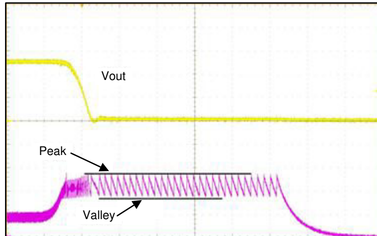
Figure 7-1. Current Limit Operation During Output Short Circuit
