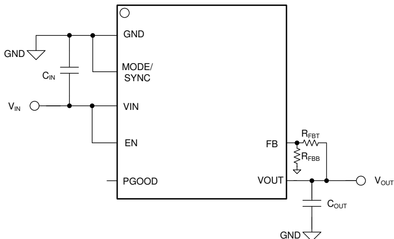
Figure 8-2. Adjustable 1.2-V to 15-V Output Typical Application Circuit
