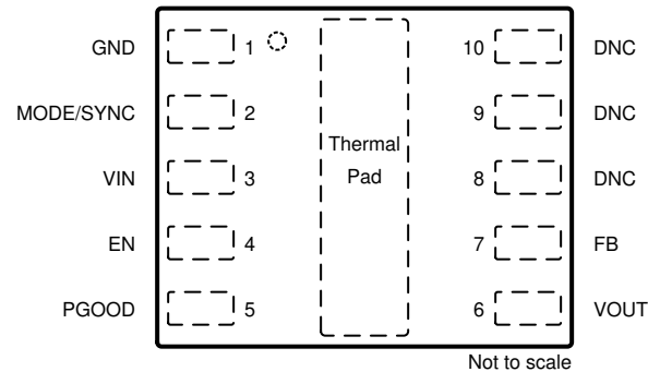
Figure 5-1. SIL 10-Pin MicroSiP™ Package Top View
