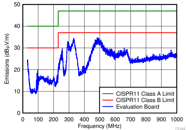
Figure 6-8. Radiated EMI
