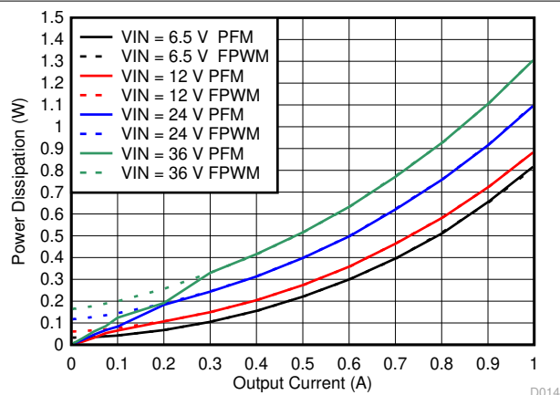
Figure 6-10. Power Dissipation
