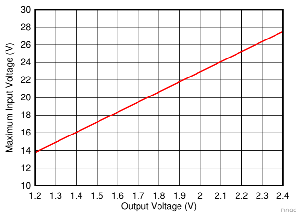
Figure 8-3. Maximum Input Voltage for V_{OUT} < 2.5 V
