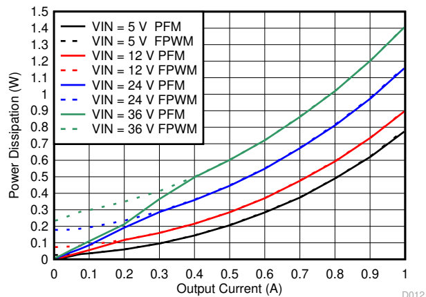
Figure 6-14. Power Dissipation
