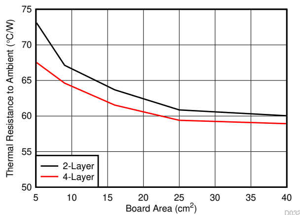
Figure 8-48. Package Thermal Resistance vs Board Copper Area
