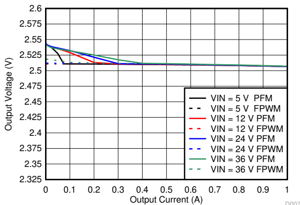
Figure 8-34. Line and Load Regulation
