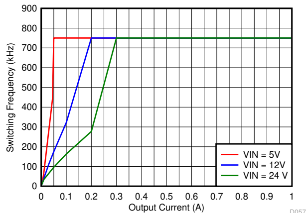
Figure 6-26. Auto PFM Mode Switching Frequency vs Output Current
