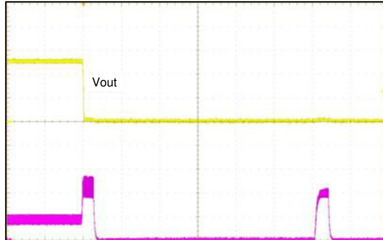
Figure 7-2. Hiccup Operation
