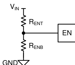
Figure 8-5. Enable Divider to Set External UVLO Threshold
