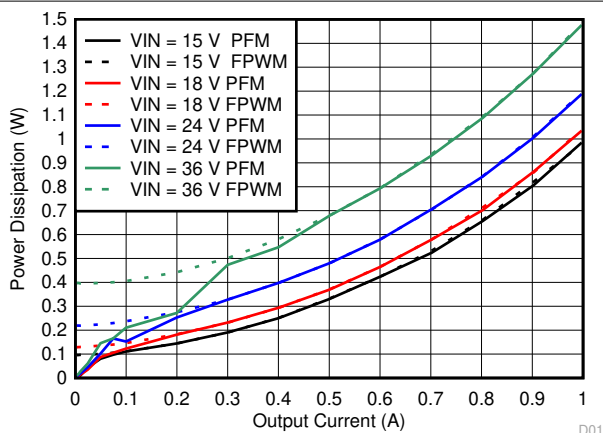
Figure 6-11. Power Dissipation
