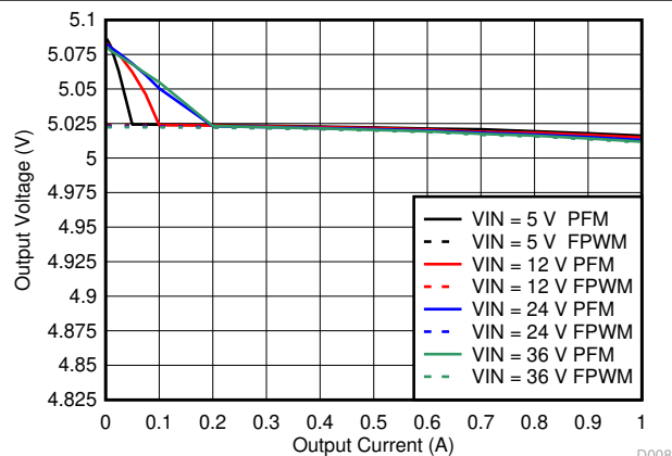
Figure 8-10. Line and Load Regulation
