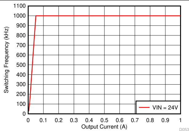
Figure 6-28. Auto PFM Mode Switching Frequency vs Output Current
