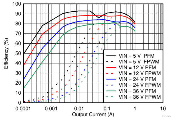
Figure 8-12. Efficiency
