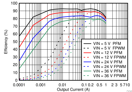
Figure 8-43. Efficiency for V_{OUT} = 3.3\text{ V}
