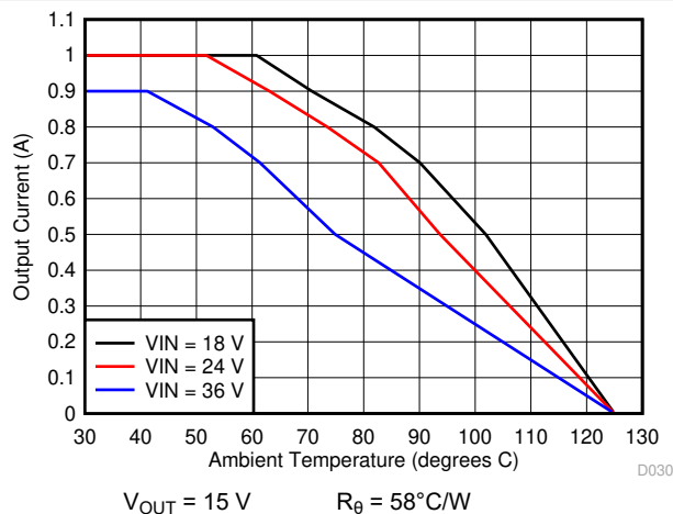
Figure 6-23. Ambient Temperature vs Output Current
