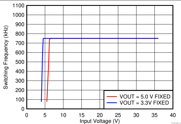
Figure 6-32. Switching Frequency vs Input Voltage for Fixed Output Options at Full Load
