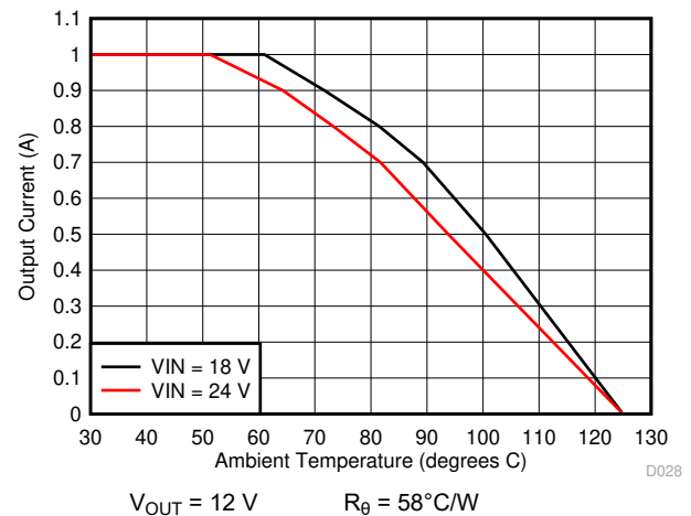
Figure 6-22. Ambient Temperature vs Output Current
