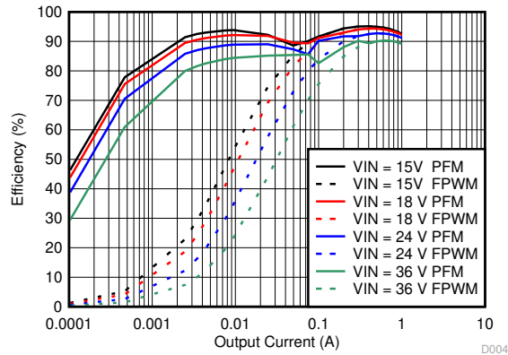
Figure 8-18. Efficiency
