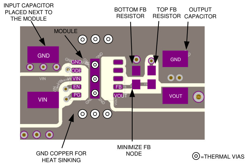
Figure 8-50. Layout Example With Adjustable Output Version
