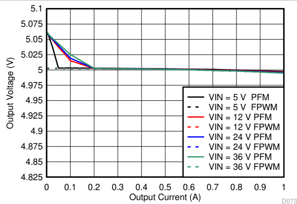
Figure 8-44. Line and Load Regulation for V_{OUT} = 5\text{ V}
