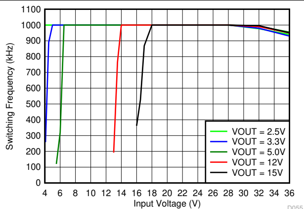
Figure 6-31. Switching Frequency vs Input Voltage for Adjustable Output Options at Full Load
