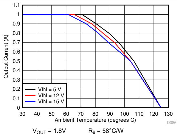
Figure 6-18. Ambient Temperature vs Output Current
