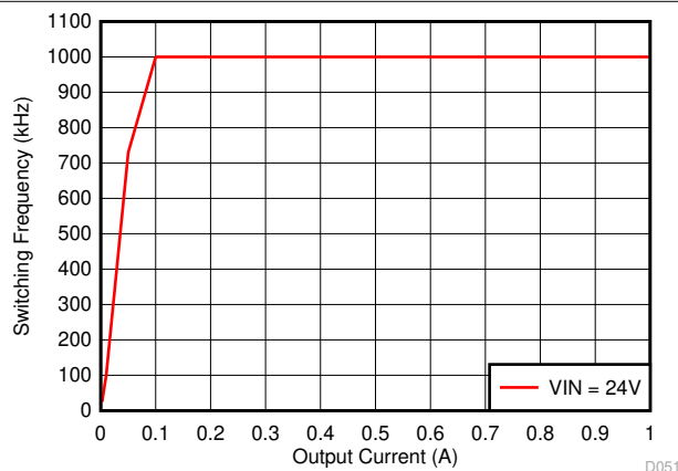
Figure 6-29. Auto PFM Mode Switching Frequency vs Output Current
