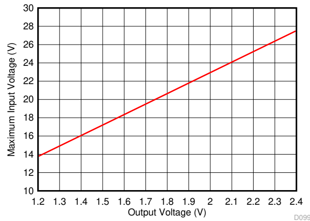
Figure 9-3. Maximum Input Voltage for V_{OUT} < 2.5 V
