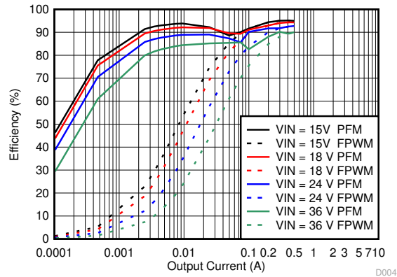
Figure 9-18. Efficiency
