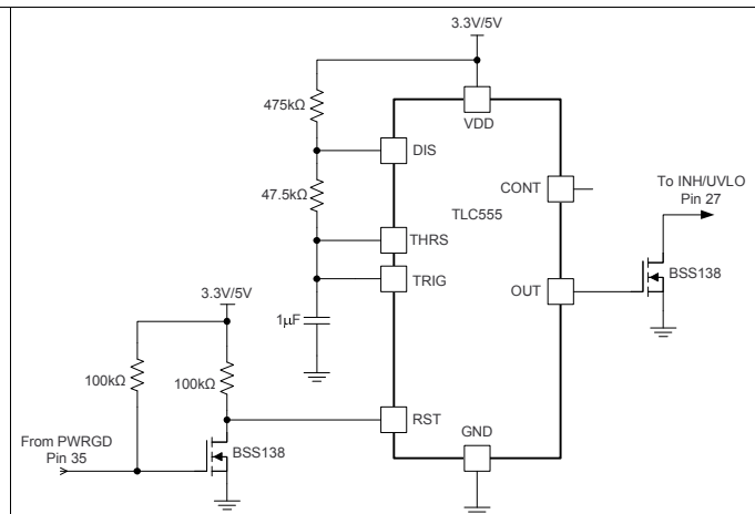
Figure 37. Over-Current Protection Circuit
