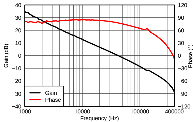
Figure 10. V_{OUT}=1.8\text{ V} , I_{OUT}=3\text{ A} , C_{OUT1}=100\text{ }\mu\text{F} ceramic, C_{OUT2}=100\text{ }\mu\text{F} ceramic, f_{SW}=480\text{ kHz}
