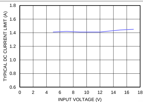
Figure 65. Typical Current Limit V_{OUT} = 3.3 V, T_A = 85 °C
