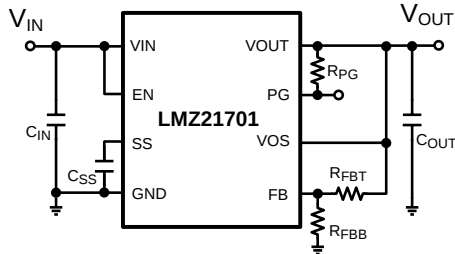
Figure 56. Typical Applications Circuit
